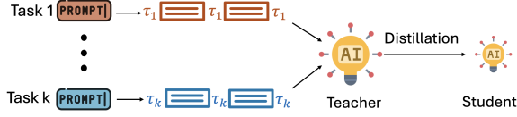
Figure 2: Positional Task Conditioning. Task tokens (\tau_1, \dots, \tau_k) are inserted at structural boundaries within each prompt: before the introduction, before the input data, and at the end. The teacher LLM data is generated using these task tokens and used to distill the student LLM.
