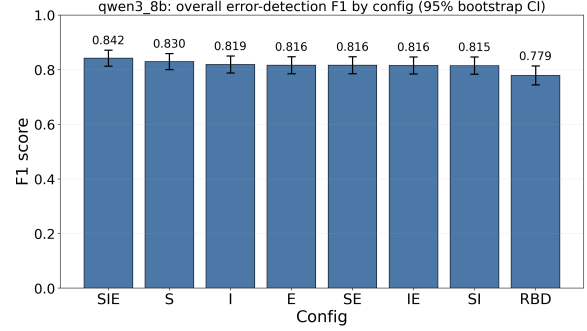
Figure 4: F1 scores across 7 positional configurations on Qwen3 8B with 95% bootstrap CI. S = start of prompt, I = before input, E = end of prompt. The optimal configuration (SIE) places task tokens at the start, input, and after the end of the prompt, achieving 84.2% F1. All PTC configurations outperform RBD (77.9%).
