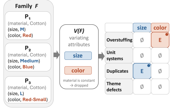
Figure 3: Divide-and-conquer on a t-shirt family F : we extract the varying attributes V(F) (dropping the constant material) and classify each (task, attribute) pair independently as no error ( \phi ), non-egregious (NE), or egregious (E). Two egregious defects are detected in this example: Overstuffing on color and Duplicates on size.
