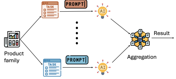
Figure 1: The figure depicts our divide and conquer approach. We take a product family as input and decompose each of its varying attributes (§3.1) into multiple classification tasks. Each task has its own prompts; the results are aggregated for the family.
