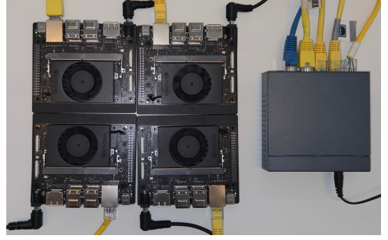
Fig. 4. Physical testbed used to evaluate PrivPair. With PrivPair, edge devices such as the NVIDIA Jetson Orin Nano can serve as clients in FL-based LLM fine-tuning.
