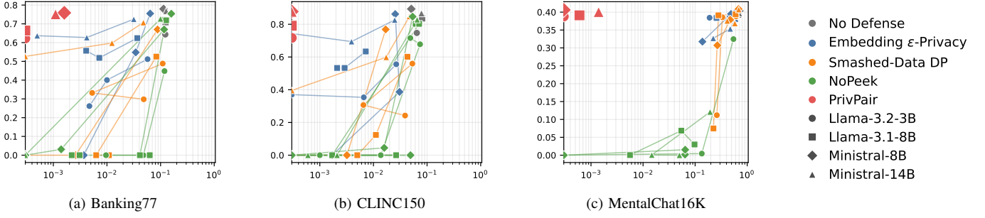
Fig. 7. Privacy-utility landscape of the scanned baseline scales, No Defense, and PrivPair. The horizontal axis is Direct Forward ROUGE-1 at the final checkpoint, shown on a log scale. The vertical axis is task utility. The top left is better, with lower leakage and higher utility.
