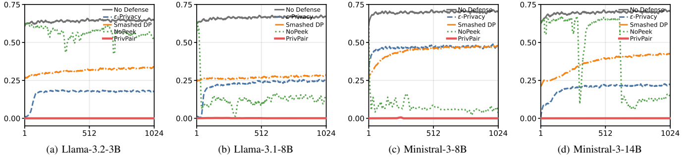
Fig. 5. Sixteen-step moving mean Direct Forward ROUGE-1 on MentalChat16K throughout training under different defense conditions.
