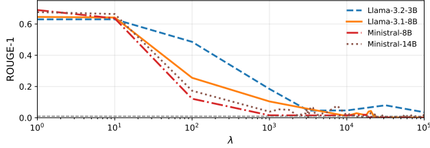
(c) NoPeek
