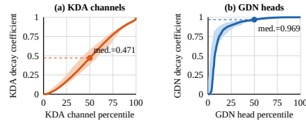
Figure 2: Weight-only decay profiles for KDA and GDN.
