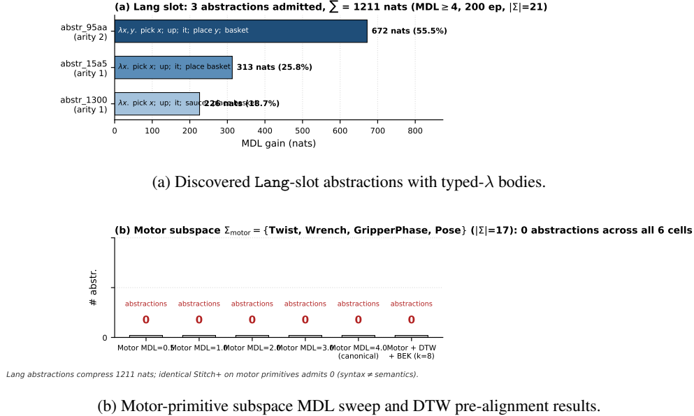
Figure 6: Library learning panel. Top: language abstractions. Bottom: motor subspace sweep.
