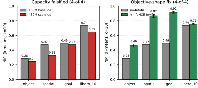
Figure 3: Twin claim: capacity vs. objective shape. Left: 430M Phase C regresses on 4-of-4 suites (red) at fixed objective. Right: adding the auxiliary InfoNCE term to the 188M Phase A objective lifts 4-of-4 suites (green) at fixed capacity.
