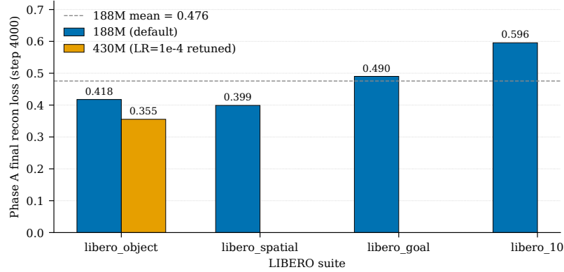
Phase A world-model warmup: per-suite final reconstruction loss (188M baseline vs. 430M LR-retuned on libero_object)
