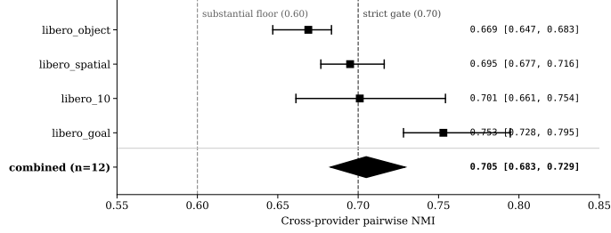
Figure 5: Forest plot of cross-provider seed convergence at n=12 pairs. Per-suite point estimates with n=3 bootstrap intervals; combined diamond = 0.705, 95% CI [0.683, 0.729]. Dashed lines: 0.70 strict gate, 0.60 substantial floor. The combined CI is borderline against 0.70 and robustly above 0.60.
