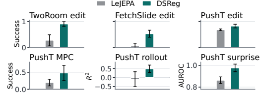
Figure 4: DSReg improves all six sparse-use probes. DSReg in teal, LeJEPA in gray. Tasks are (1) editing (top) and (2) control, prediction, and monitoring (bottom).
