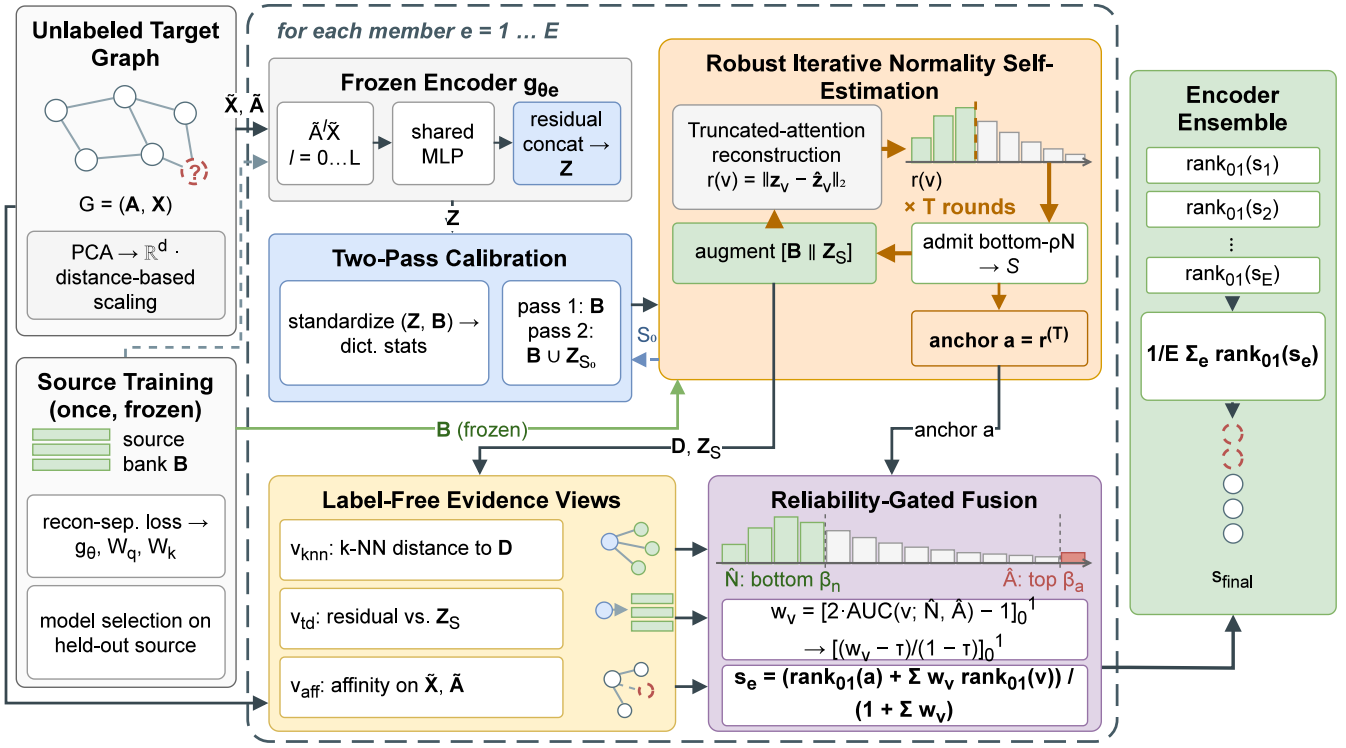
Figure 1: Overview of RINSE. For each ensemble member, the encoder g_{\theta_e} , attention projections \mathbf{W}_q, \mathbf{W}_k , and source bank B_e are learned or constructed from source graphs and then frozen. All target-time components operate independently on the unlabeled target graph, without labels, gradients, or per-target tuning. The blue dashed path supplies provisional normals S_0 to the second calibration pass; red dashed nodes denote suspected anomalies ranked highest at output.
