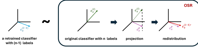
Fig. 2: Reversing the Transition Within the Output Space to Remove An Existing Label
