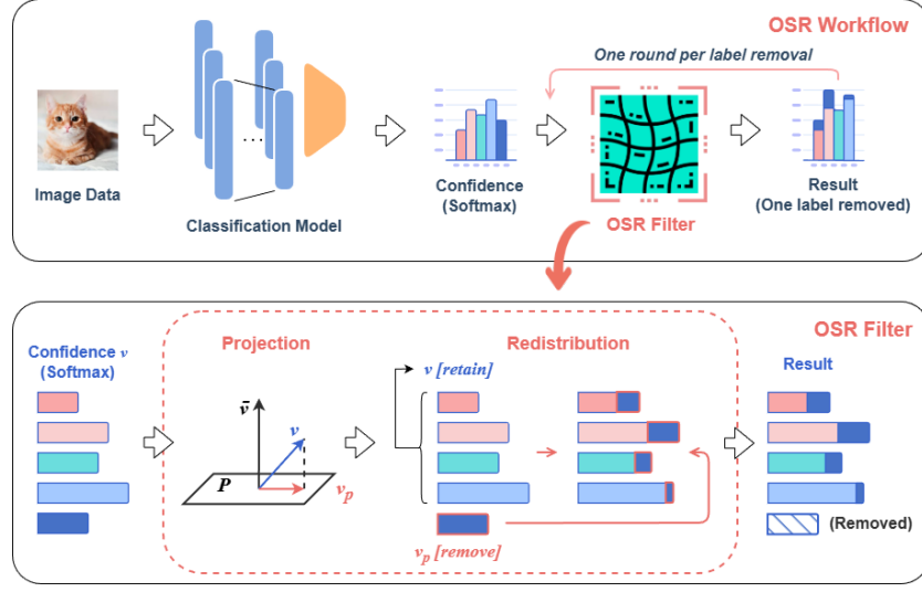
Fig. 3: Overview of our OSR filter, which applies a post-hoc output-space redistribution comprising a projection step and a redistribution step. It removes the influence of the removed labels, reweights the remaining labels, and reassigns the residual probability mass associated with the removed labels, using a classifier trained on the updated label set as reference. This adjustment revises the original predicted confidence while preserving semantic consistency.
