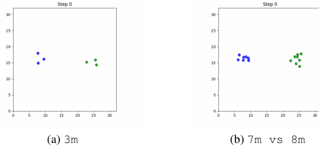
Figure 10: SMAX
