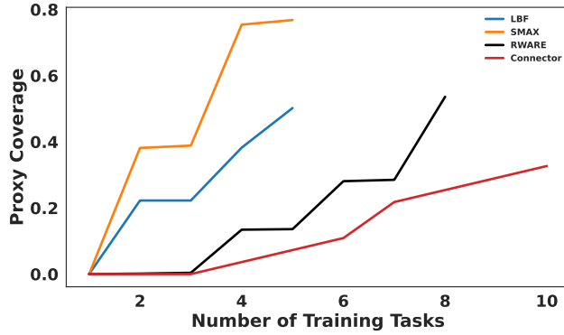
Figure 6: Proxy coverage metric for each environment’s test set. This proxy metric, based on the similarity between test and training tasks, provides insight into how performance is likely to improve as additional training tasks are included.
