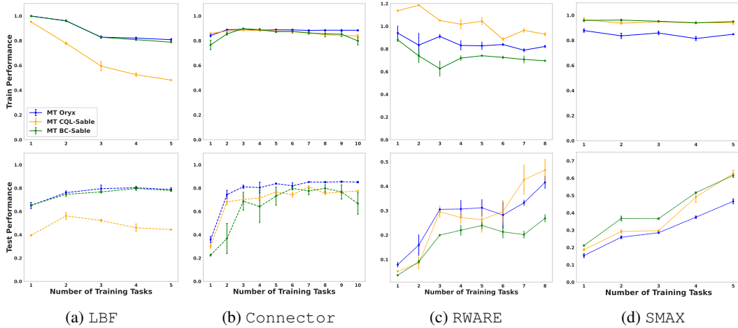
Figure 4: The effect of increasing task diversity on performance. Top: training tasks. Bottom: held-out test tasks. When training on a single task, performance is high on the training task but generalisation to held-out tasks is poor. As the number of training tasks increases, test-task performance steadily improves across all environments.
