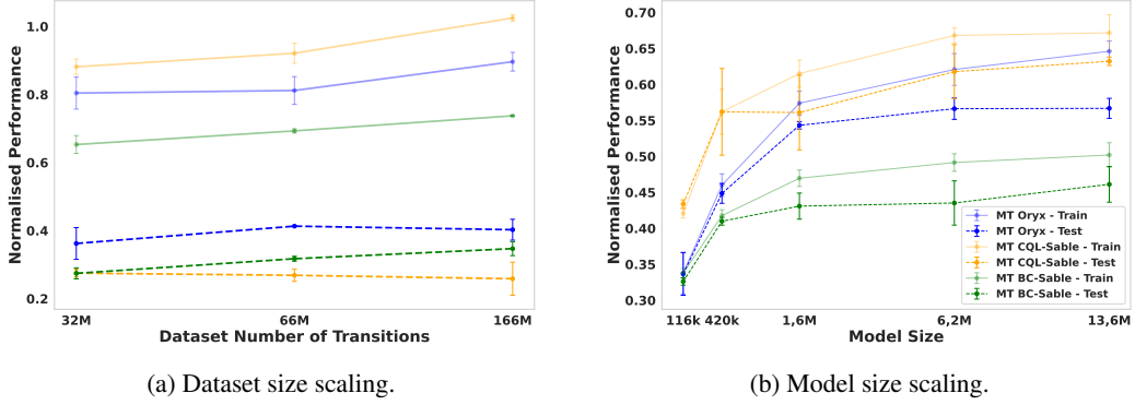
Figure 5: The impact of scaling up dataset (left) and model size (right). Fixing the number of RWARE tasks while increasing the number of transitions in the dataset leads to improved training performance, though test performance plateaus. Conversely, fixing the dataset size and varying the model size reveals a clear scaling trend, both training and test performance improve as the model grows.
