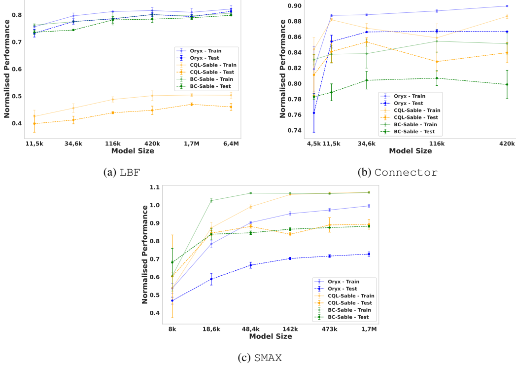
Figure 12: Performance of MT-Oryx, MT-CQL-Sable, and MT-BC-Sable on LBF, Connector, and SMAX with different model sizes. Both train and test performance of all algorithms improve with increasing model size up to a critical threshold, beyond which performance plateaus.
