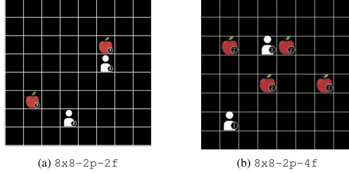
Figure 7: LBF
