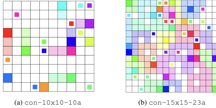
Figure 8: Connector
