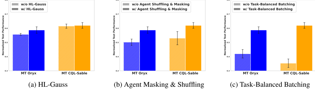
Figure 15: Ablation studies. Left: Using HL-Gauss improves test performance for MT Oryx by \approx 8\% , while the effect on MT CQL-Sable is marginal. Middle: Disabling agent masking and shuffling reduces test performance by \approx 16\% on average for both algorithms. Right: Removing task-balanced batching has the highest impact with \approx 37\% drop in test performance on average for both MT Oryx and MT CQL-Sable.
