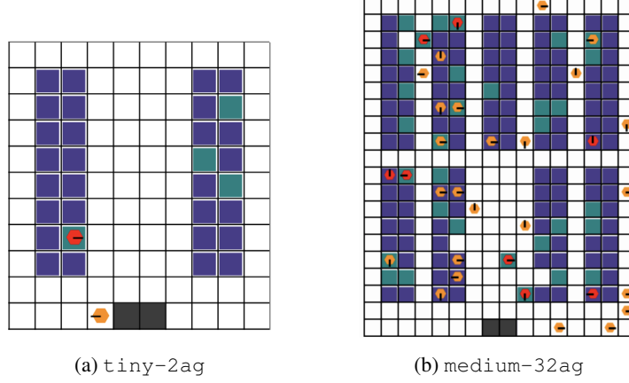
Figure 9: RWARE
