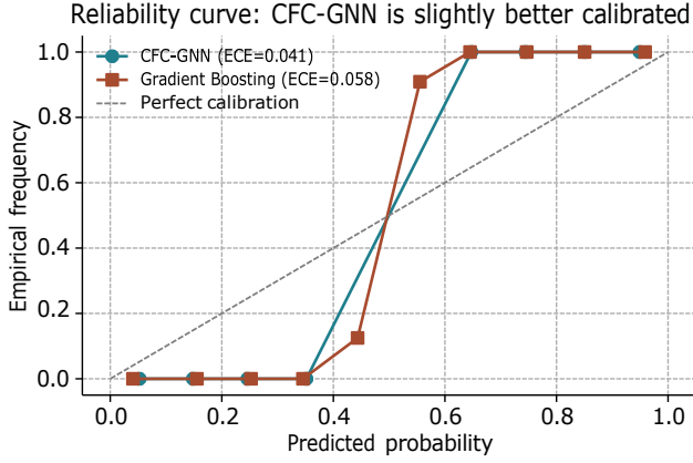
Fig. 9: Reliability curves. CFC-GNN sits closer to the diagonal, especially in the mid-probability regime that a supervisor would use for a watch-list threshold.
