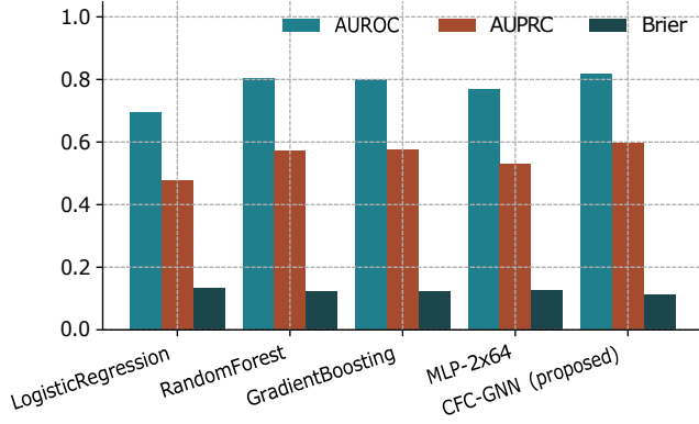
Fig. 7: Detection quality across baselines and CFC-GNN. The proposed model wins on all three metrics.
