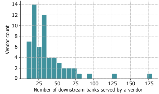
Fig. 3: Distribution of the number of downstream banks per vendor in the synthetic graph. The right tail is what makes a targeted attack on a single vendor systemically relevant.
