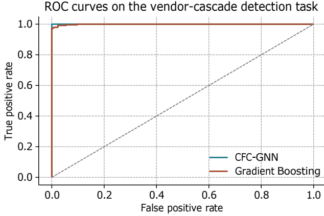
Fig. 10: ROC curves on the vendor-cascade detection task.
