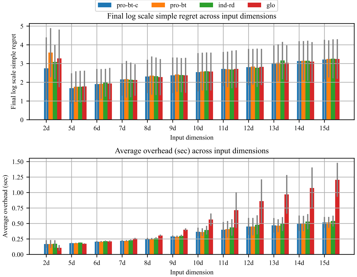
Figure 5: Performance and computational overhead on 47 synthetic benchmark functions across input dimensions 2 \leq d \leq 15 . The top plot shows the average simple regret, and the bottom plot shows the computational overhead. BO-pro-c, BO-pro, and BO-ind exhibited modest increases in overhead as dimensionality increases, whereas BO-glo exhibited a substantially steeper increase.
