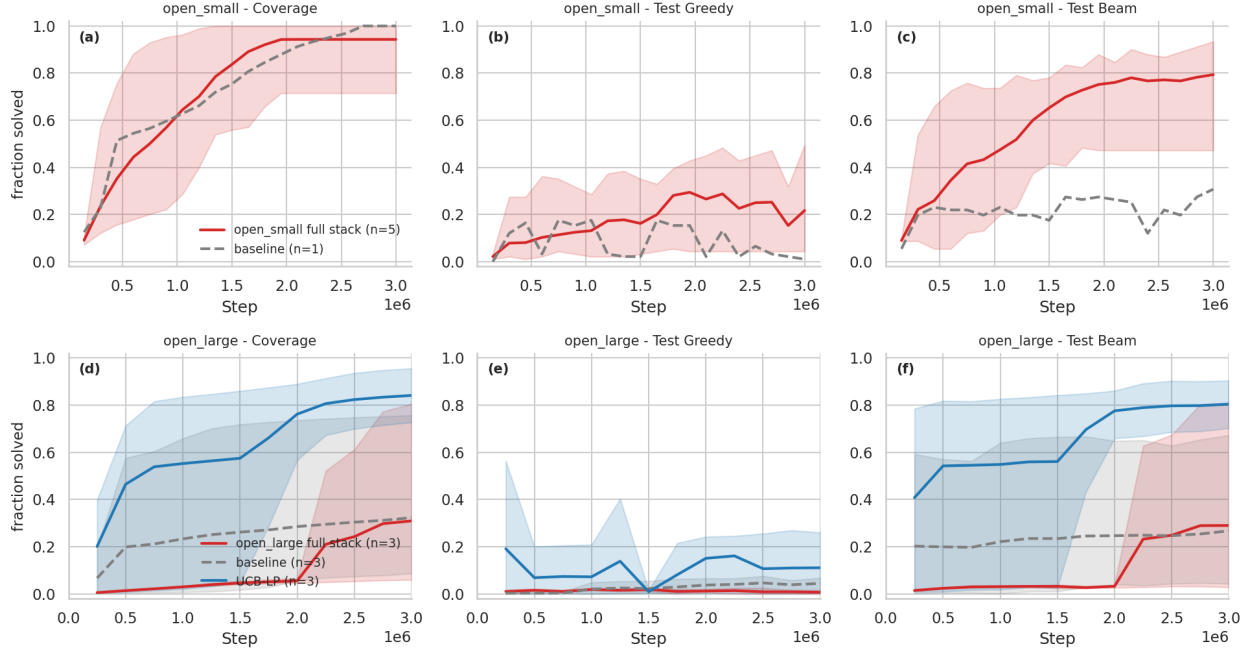
Figure 1: Open-equation learning curves (coverage, greedy and beam-width-5 test accuracy) for open_small (top) and open_large (bottom). Red: full method stack; grey dashed: baseline; blue: UCB-LP. Solid lines are seed means, bands min/max; seed counts per cohort are given in the text. Per-seed distributions are in Figure 3.
