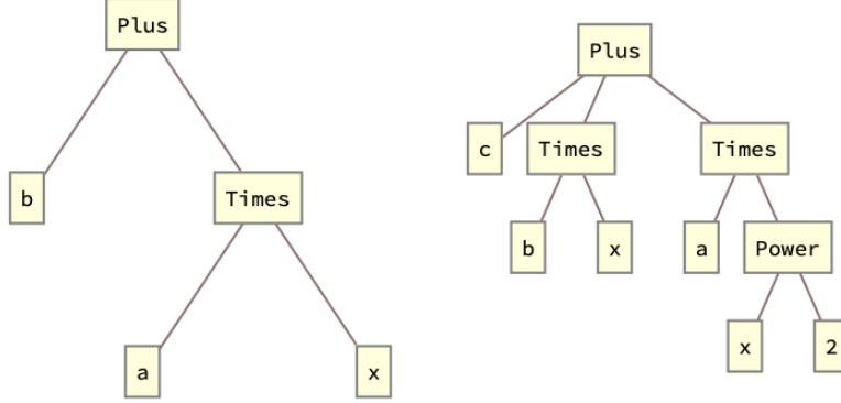
Figure 7: Expression trees for ax + b and ax^2 + bx + c . The agent’s state vector is a preorder traversal of these trees, padded to length L = 50 .
