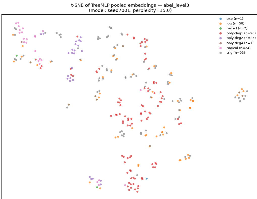
Figure 8: t-SNE projection of TreeMLP pooled embeddings for 300 small-dataset equations, colored by structural type. Clusters correspond to equation family rather than to specific coefficient assignments.
