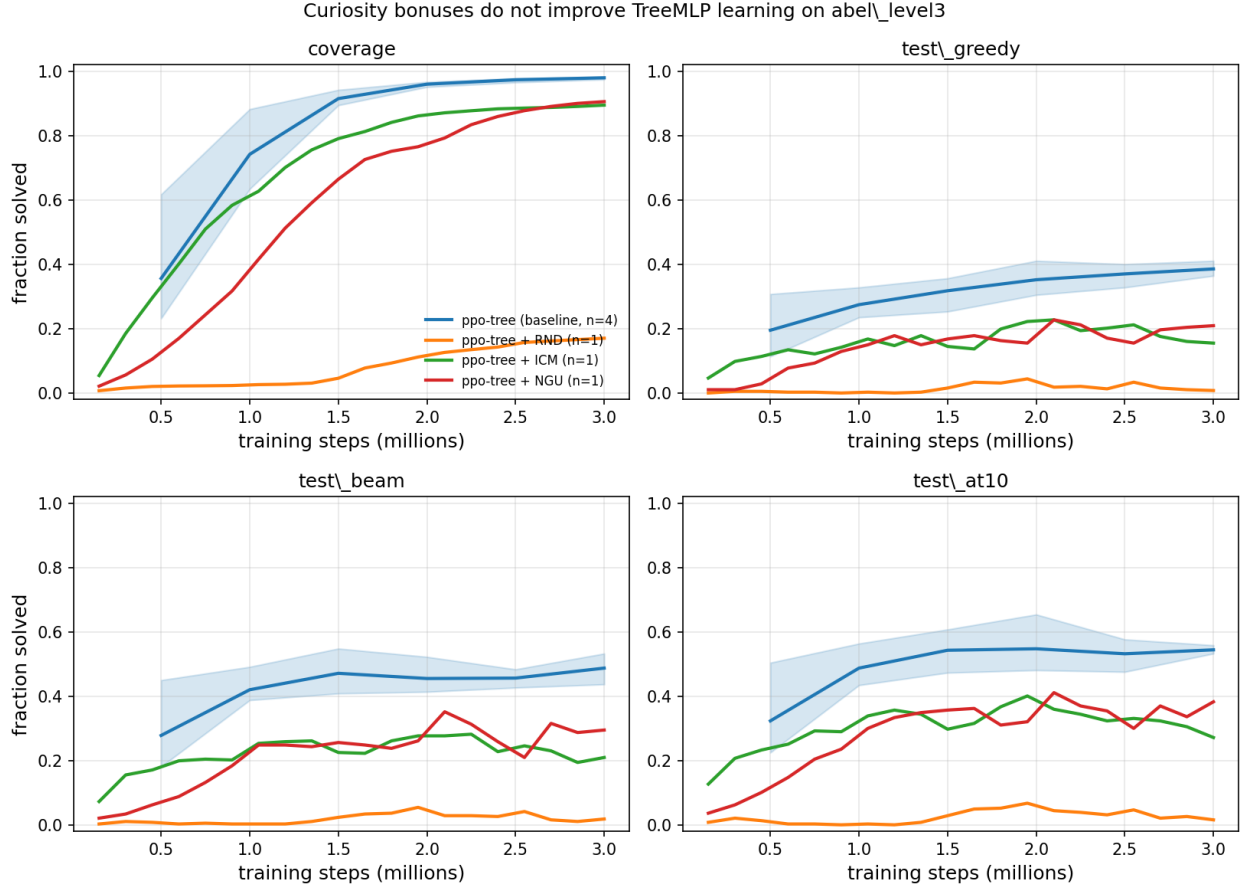
Figure 6: Curiosity bonuses (ICM, NGU, RND) do not improve TreeMLP learning on abel_level3 (single-seed bonus runs vs. an n=4 -seed no-curiosity baseline; y -axis test metrics over training steps). No bonus matches the baseline; RND fails to learn. These single-seed results are suggestive, not conclusive.
