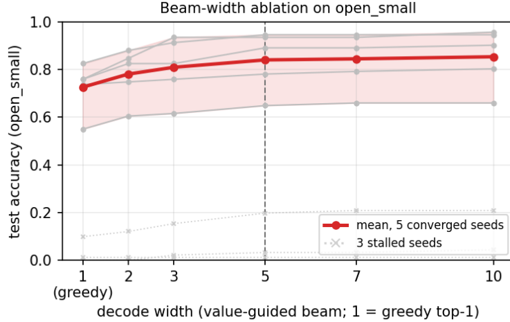
Figure 2: Beam-width ablation on open_small (cohort W, Table 2). Value-guided-beam test accuracy vs. decode width (width 1 = greedy top-1) across eight full-stack open_small checkpoints; solid grey lines are the five converged seeds, dotted the three stalled seeds (greedy \approx 0 , consistent with the seed-level bimodality of Section 4.2.5), red is the mean over the converged seeds with min-max band. On the converged seeds accuracy rises from greedy (0.73) through width 5 (0.84) and then saturates, supporting width 5 as the reported operating point; a stalled policy solves \approx 0 at every width, so beam-width is only meaningful once the policy has learned solution paths. (This is cohort W’s greedy anchor of 0.73, not the headline greedy 0.67 of cohort H: these checkpoints were trained to 5M rather than 3M steps, are a different seed draw, and are scored on the full 91-equation file rather than the 70% test slice, so they sit above cohort H in absolute level. The width-dependence shape and the high greedy anchor are the point; the levels are not comparable across cohorts.)
