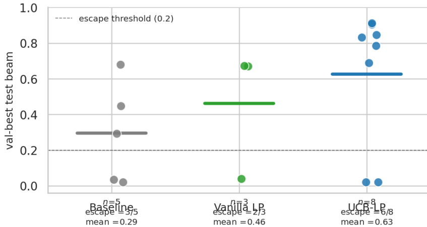
Figure 3: Per-seed val-best test beam on open_large . Each dot is one training run; horizontal bar is the cohort mean. The escape mode (beam \geq 0.2 ; escapes cluster near 0.7–0.9) is more populated and reaches higher values under UCB-LP, while the stall mode at \sim 0.02 is preserved (UCB-LP: 2/8 stalls, both from crashed seeds whose pre-crash trajectories were already stalled).
