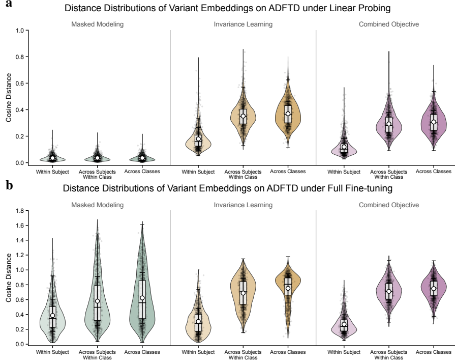
Fig. 9: Pairwise-distance analysis of pre-training objective ablation on ADFTD. a , Cosine-distance distributions of ADFTD representations under linear probing. b , Cosine-distance distributions after full fine-tuning. For each objective variant, distances are computed for segment pairs from the same subject, from different subjects within the same diagnostic class and from different diagnostic classes. Violin plots show the distribution of pairwise cosine distances, box plots summarize the median and interquartile range, and white circles with error bars indicate mean \pm s.d..
