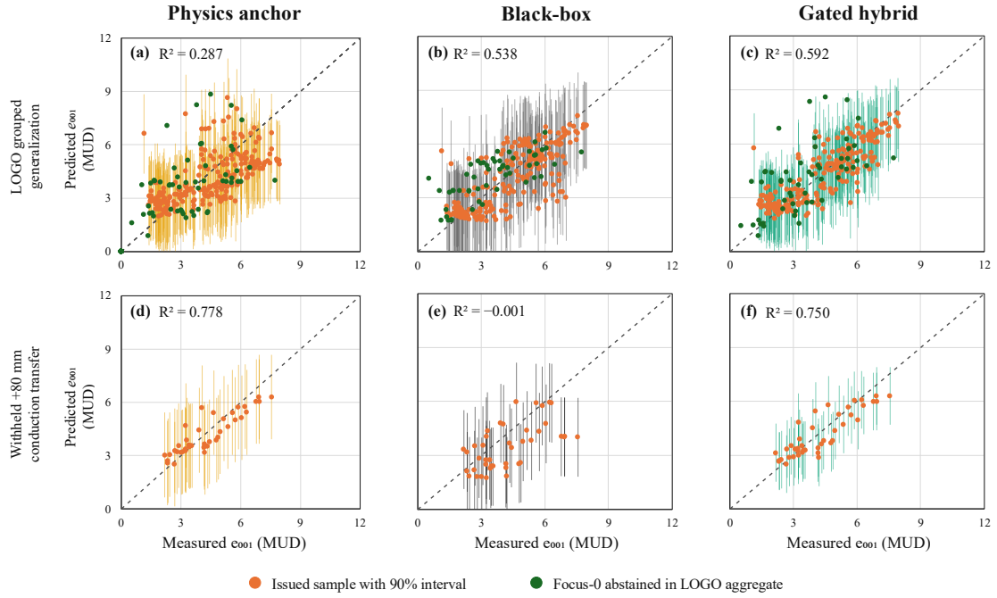
Figure 5. Regime-specific parity of measured and predicted \epsilon_{001} for the greybox anchor, black-box RF, and gated hybrid. Panels (a-c) show LOGO results; panels (d-f) show the withheld +80 mm evaluation. Dashed lines denote 1:1 agreement. Orange markers identify framework-retained observations, whereas green markers identify focus-zero observations for which the framework abstained. Vertical bars show model-specific 90% inner group-CV empirical intervals where issued. The black-box comparator does not implement abstention; its full-set UQ is reported in Table 7. All axes span 0-12 MUD.
