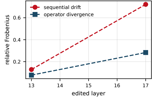
Figure 2: Sequential drift \|\Delta_{\text{proposed}} - \Delta_{\text{central}}^{\text{Alpha}}\|_F / \|\Delta_{\text{central}}^{\text{Alpha}}\|_F and operator divergence \|N_{\text{all}} - N_G\|_F / \|N_G\|_F increase monotonically across the edited layers (13–17), peaking at the last; five-layer means 0.4547 and 0.1879. Markers show the layer-13 and layer-17 endpoints.
