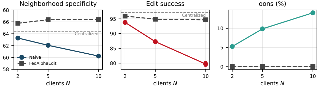
Figure 1: The naive combination and FedAlphaEdit as the same total workload (5000 edits) is partitioned across a growing number of clients N : neighborhood specificity (left), edit success (middle), and oons (right; the FedAlphaEdit series is at the measurement floor throughout). Dashed lines mark the centralized reference (64.43 and 97.08). All points are three-seed mean \pm SD. The per-client edit count co-varies with N (Section 4.2).
