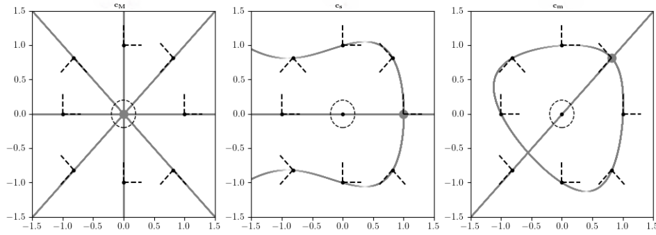
Figure 6: Tangency sets of h in (1.43) relative to different critical points. The tangency arcs may break the symmetry of the reference critical point. Any critical point lying on an arc has at least the symmetry of that arc.
