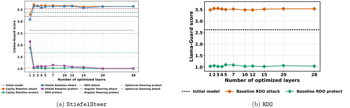
Figure 3: Effect of the number of rotated layers L on DeepSeek-R1-7B, in both regimes, measured by the mean Llama-Guard score on the 1 to 4 scale. Dimensionality of rotation is n = 35 .
