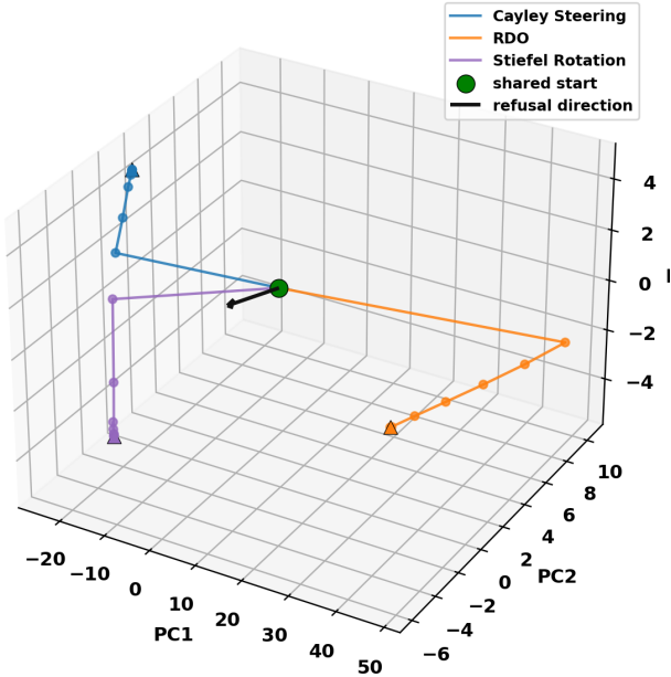
Figure 4: Trajectories of the residual-stream activation at the intervened layer of DeepSeek-R1-7B, projected onto its first three principal components.
