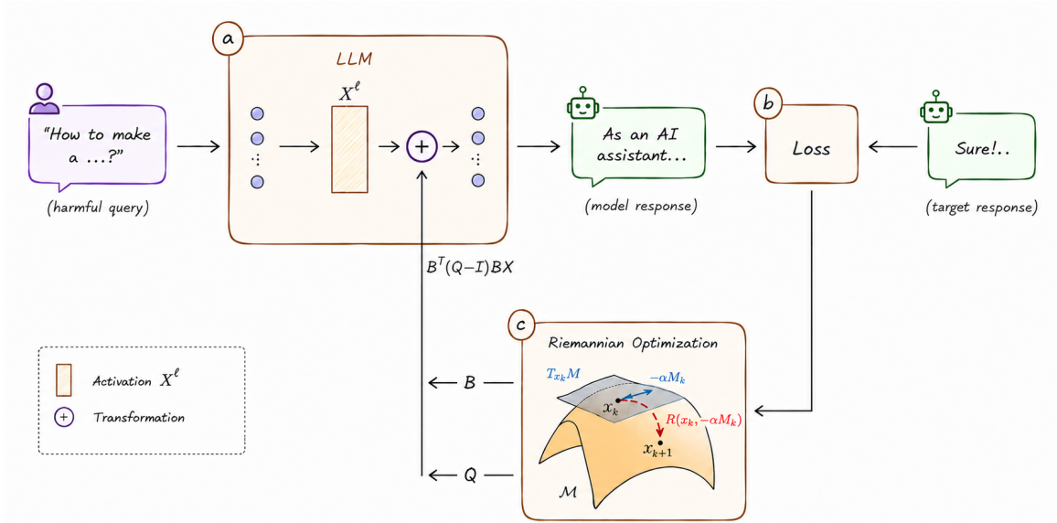
Figure 1: Principal scheme of StiefelSteer . It consists of: (a) parameter-efficient rotation of activations in selected layers, parameterized via matrices B and Q ; (b) computation of the cross-entropy between the expected and observed model outputs; (c) computation of updates via Riemannian gradients of the loss; and (d) optimization of B and Q to induce a more effective rotation.
