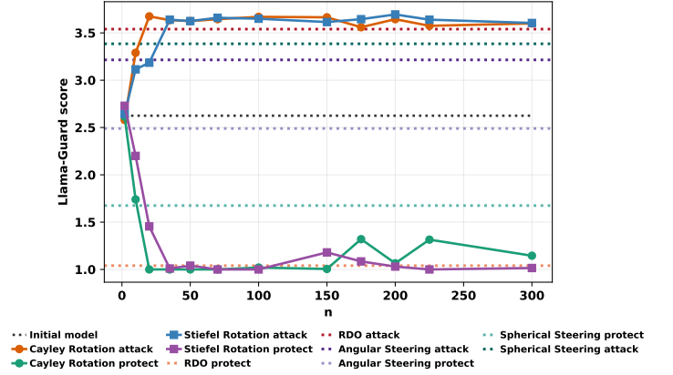
Figure 2: Effect of the rotation subspace dimension n on DeepSeek-R1-7B, in both the attack and the defensive regime, measured by the mean Llama-Guard score on the 1 to 4 scale. All layers rotated.
