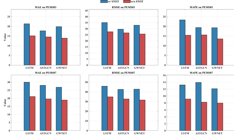
Figure 7: Mask pre-training component ablation on PeMS03 and PeMS07.
