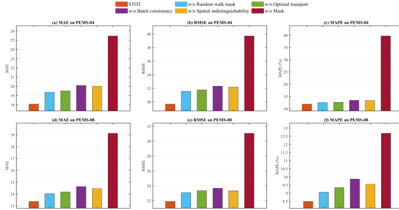
Figure 4: Mask pre-training component ablation on PeMS04 and PeMS08.
