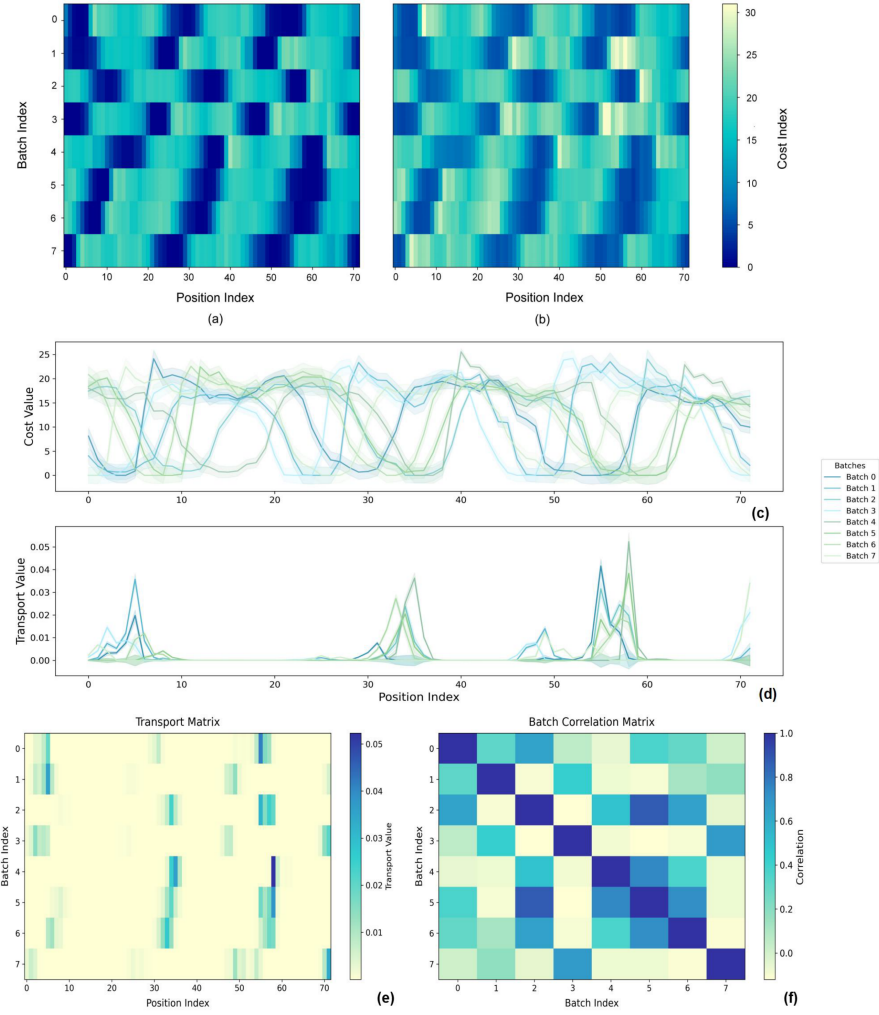
Figure 10: Visualization of OT and batch consistency: (a) and (b) cost matrices before and after batch consistency for the first 72 timesteps (6 patches), (c) and (d) the final cost matrix and OT matrix, (e) transport-matrix heatmap, and (f) batch-mask correlation matrix showing the effect of batch consistency on mask generation.
