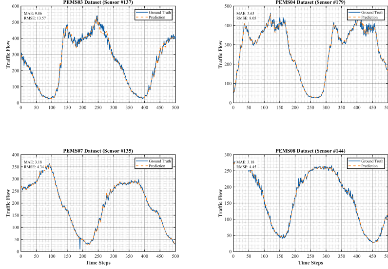
Figure 6: STOT forecasting visualization on four datasets after pre-training.
