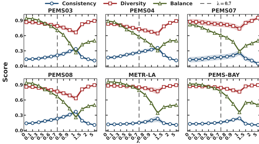
Figure 11: Consistency, diversity, and balance scores as functions of the batch consistency weight \lambda on the six datasets. The dashed line marks the default \lambda = 0.7 .
