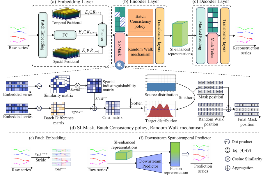
Figure 1: Architecture of STOT: (a) the embedding layer aggregates raw long-term traffic data with temporal and spatial positional features; (b) the encoder learns spatially indistinguishable node representations through masked reconstruction; (c) the decoder reconstructs masked positions from SI-enhanced representations; (d) mask generation uses SI-Mask, Batch Consistency, and Random Walk, where SI-Mask guides spatial indistinguishability and the latter two constrain representation continuity and richness; (e) patch embedding segments spatiotemporal data into local-pattern units; and (f) the STOT-enhanced downstream predictor can be integrated with various downstream architectures.
