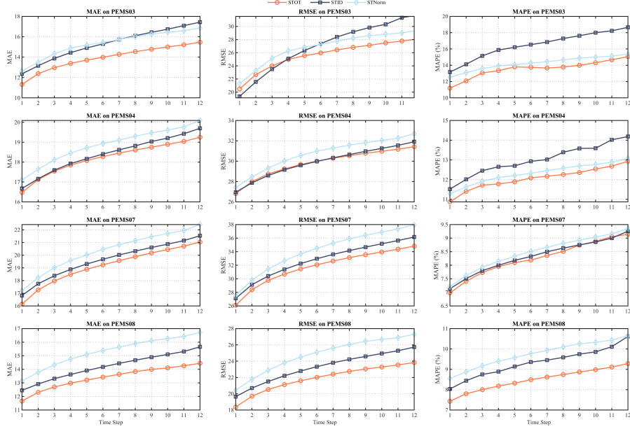
Figure 3: Multi-step prediction comparison on PeMS03, PeMS04, PeMS07, and PeMS08.
