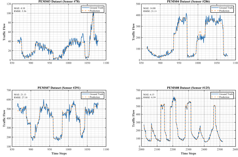
Figure 5: STOT reconstruction visualization on four datasets during pre-training.
