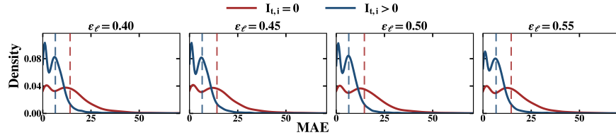
Figure 2: KDE distributions of node-sample forecasting MAE grouped by the spatial indistinguishability score in Equation 5. Dashed lines indicate the group-wise mean MAE.
