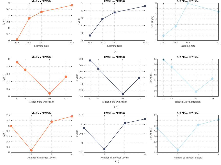
Figure 8: STOT parameter sensitivity on PeMS04 under MAE, RMSE, and MAPE.
