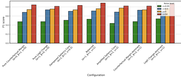
(a) Performance (F1 score)
