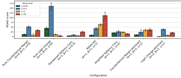
(b) Explainability (ROAD score)
