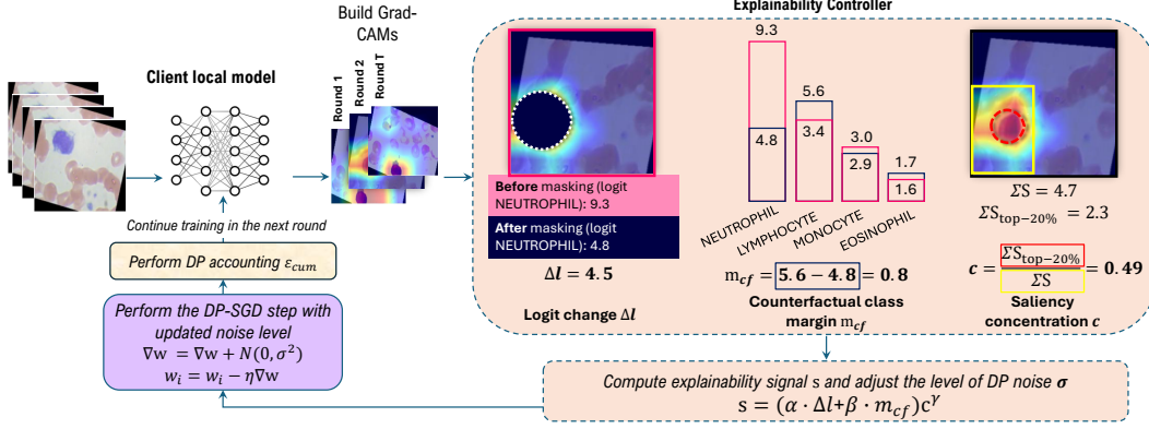
Figure 1: Overview of FL client’s training procedure. The adaptive training process repeats for T iterations for each client.
