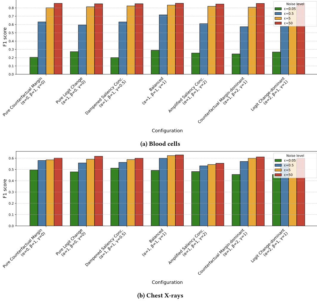
Figure 7: Ablation analysis of signal component weights on predictive performance (F1 score) across noise levels ( \epsilon ). Each configuration (Table 5) varies the weights of the logit change ( \alpha ), counterfactual margin ( \beta ), and saliency concentration ( \gamma ) components.
