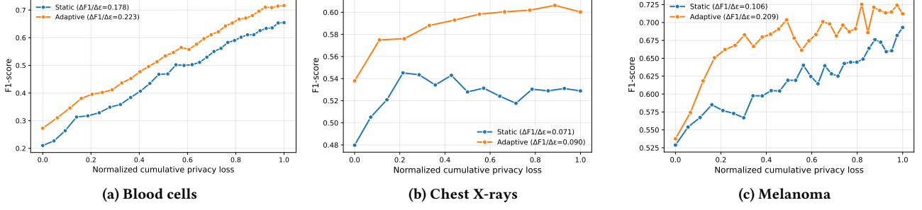
Figure 4: Privacy-utility efficiency of global FL models across datasets, comparing FL+DP training with static DP noise and our adaptive XCal-FL training ( \epsilon = 0.5 with \alpha = \beta = \gamma = 1 ). Efficiency is defined as the ratio of F1 score to the cumulative privacy loss.
