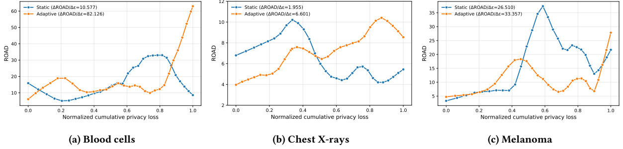
Figure 5: Privacy-explainability efficiency for global FL models across datasets, comparing FL+DP training with static DP noise and our adaptive XCal-FL training ( \epsilon = 0.5 with \alpha = \beta = \gamma = 1 ). ROAD curves were smoothed using LOWESS smoothing. Efficiency is defined as the ratio of ROAD score to the cumulative privacy loss.
