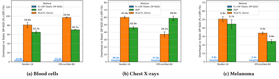
Figure 9: Per-client training overhead (%) relative to standard static DP-SGD, measured across three medical imaging datasets and two model architectures: ResNet-18 ( P=11.7M ) and EfficientNet-B0 ( P=5.3M ). Experiments were conducted on a NVIDIA’s RTX 2080 Ti GPU machine. Wall-clock per-client times (seconds), averaged over three runs, are annotated above each bar; error bars denote the standard deviation across rounds.
