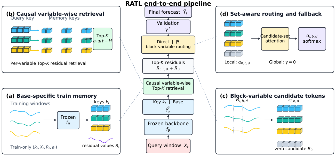
Figure 1: Overview of RATL. The center shows the end-to-end pipeline from an input window to the final corrected forecast; (a) a frozen base forecaster constructs a train-only key–residual memory; (b) Top- K residuals are retrieved independently for each variable under the temporal-availability constraint; (c) candidate trajectories are split into block–variable tokens and augmented with a zero-residual candidate; (d) J5 predicts candidate weights through set attention. Direct similarity weighting is the non-parametric baseline and uses the raw correction with \gamma = 1 ; for RATL, the correction-strength hyperparameter \gamma is selected on validation before one-shot test evaluation.
