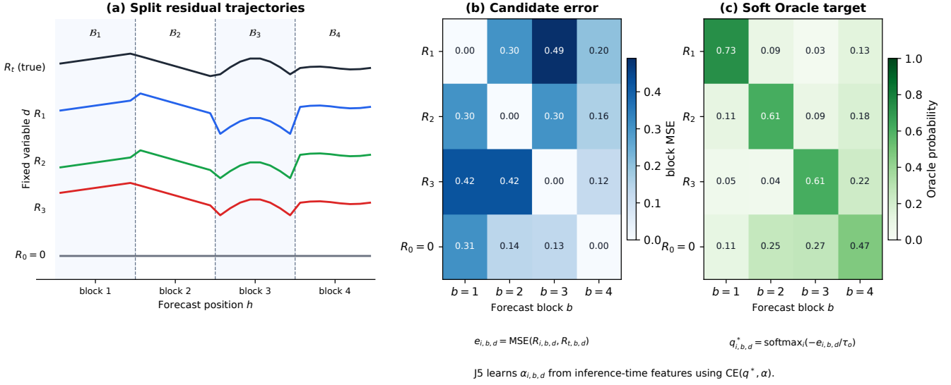
Figure 2: Construction of block-residual candidates and the soft Oracle supervision target for a fixed variable d . Full residual trajectories are first divided into consecutive temporal blocks along the forecast horizon. In each block, every historical candidate and the zero-residual candidate R_0 = 0 are compared with the current true residual to obtain the block-variable error e_{i,b,d} . A temperature-scaled softmax over negative errors then gives the teacher distribution q_{i,b,d}^* . Curves and values in the figure illustrate the procedure and are not experimental results.
