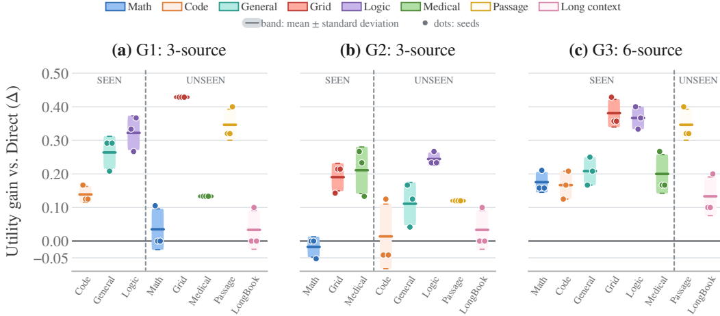
Figure 5: Generalization beyond policy-training domains. We report utility gains for policies trained on G1 (Code, General Reasoning, and Logic Games), G2 (Math, Grid Puzzles, and Medical QA), or their union G3. Passage and LongBook QA are unseen by all 3 groups. Bands and dots show the mean \pm std and individual results over three training runs.
