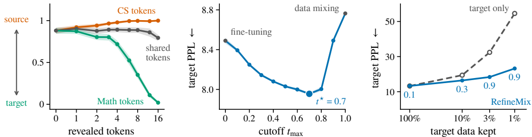
(a) More tokens settle the domain. (b) The best cutoff lies in between. (c) Scarcer target, larger gain.
