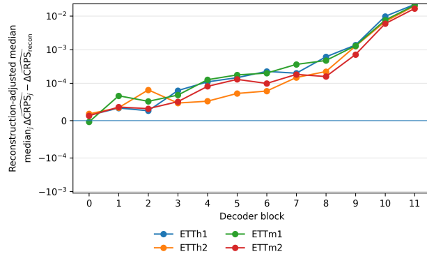
Figure 8: Reconstruction-adjusted median intervention effect from Equation 21. Values remain close to zero in early blocks and increase sharply in blocks 9–11 across all four datasets.
