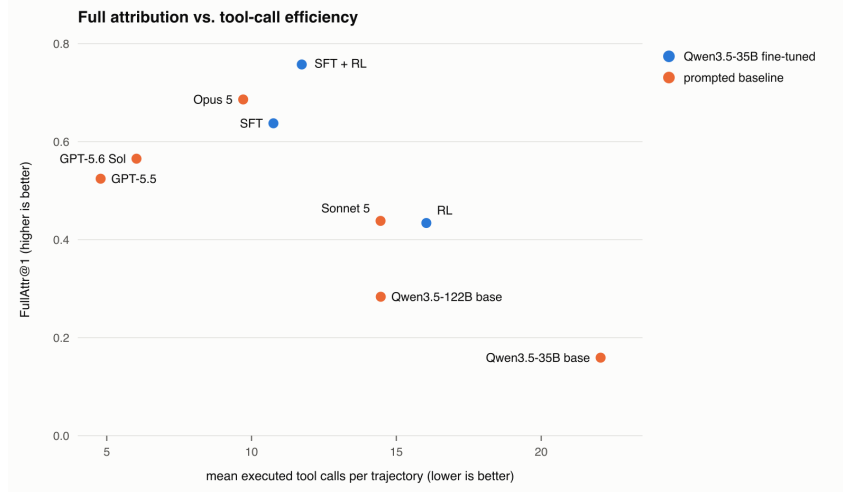
Figure 2: FullAttr@1 versus mean executed tool calls per evaluation trajectory. Each trajectory entry corresponds to one executed Python-tool call, including unsuccessful calls. Blue points denote fine-tuned Qwen3.5-35B variants, and orange points denote prompted baselines. Better performance lies toward the upper left.
