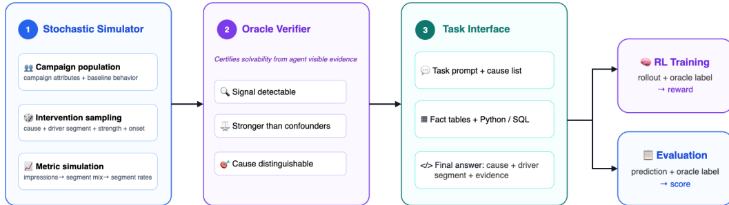
Figure 1: Overview of the TRACE workflow.
