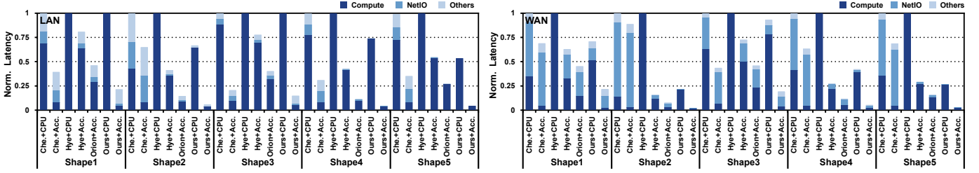
Fig. 14. Micro benchmark evaluation of linear layers.
