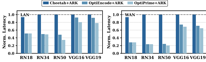
Fig. 18. Normalized end-to-end latency evaluation when integrated with ARK [41].
