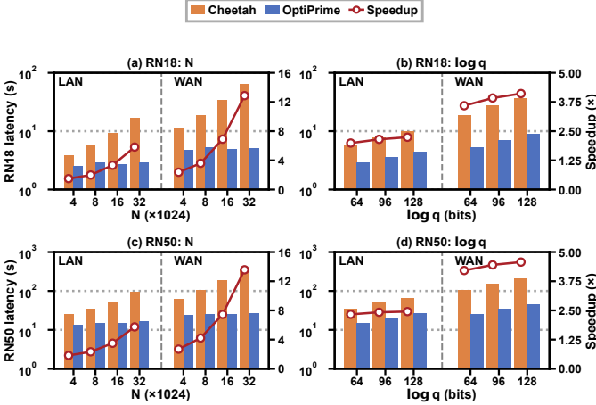
Fig. 22. HE-parameter sensitivity on ResNet-18 (a–b) and ResNet-50 (c–d) under different polynomial degrees N and ciphertext moduli q .
