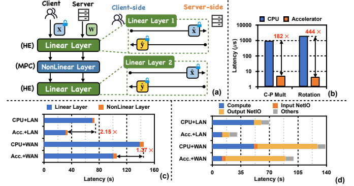
Fig. 1. (a) Hybrid HE-MPC framework. (b) Latency reduction of HE operations with the hardware accelerator. (c) Latency breakdown of ImageNet-scale ResNet50 under different network and computation conditions. "Acc." means the accelerator. (d) Latency breakdown of the Linear layer of ResNet50. "Compute" represents the HE computation. "Input NetIO" and "Output NetIO" represent the server-client network transmission of the input ciphertexts and the output ciphertexts, respectively. "Others" represents other CPU overhead, like ciphertext decryption.
