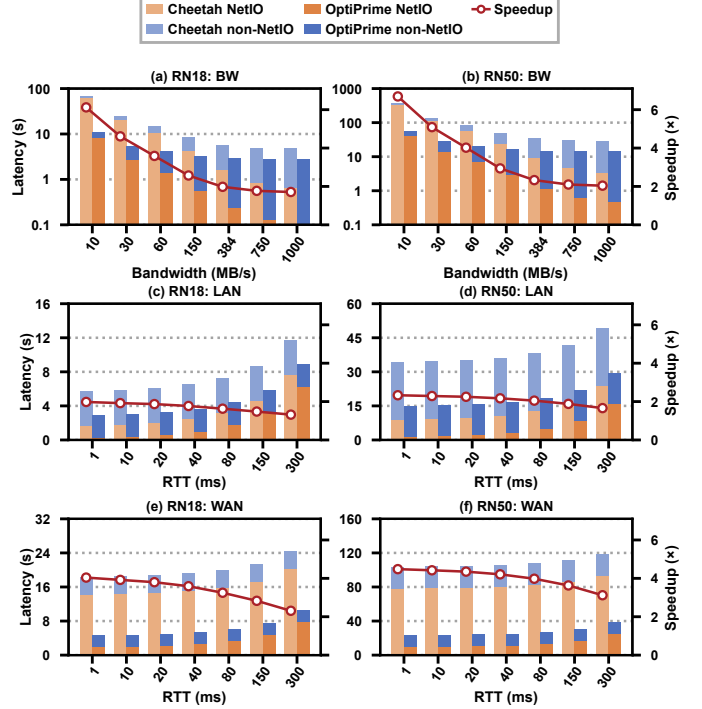
Fig. 20. Network sensitivity for ResNet-18 (left) and ResNet-50 (right): bandwidth at 1 ms RTT (top), RTT at LAN bandwidth (middle), and RTT at WAN bandwidth (bottom). Bars show NetIO/non-NetIO latency for Cheetah and OptiPrime; lines show speedup.
