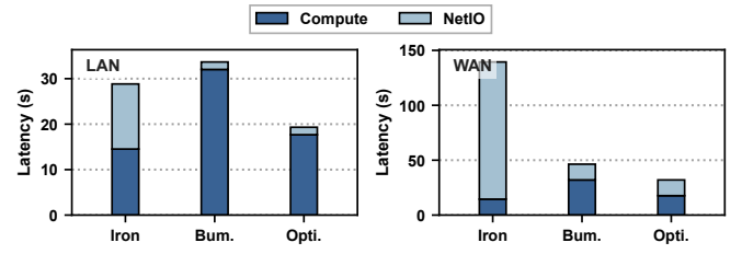
Fig. 19. Whole-network linear-layer latency on BERT-base for Iron, BumbleBee (Bum.), and OptiEncode (Opti.).
