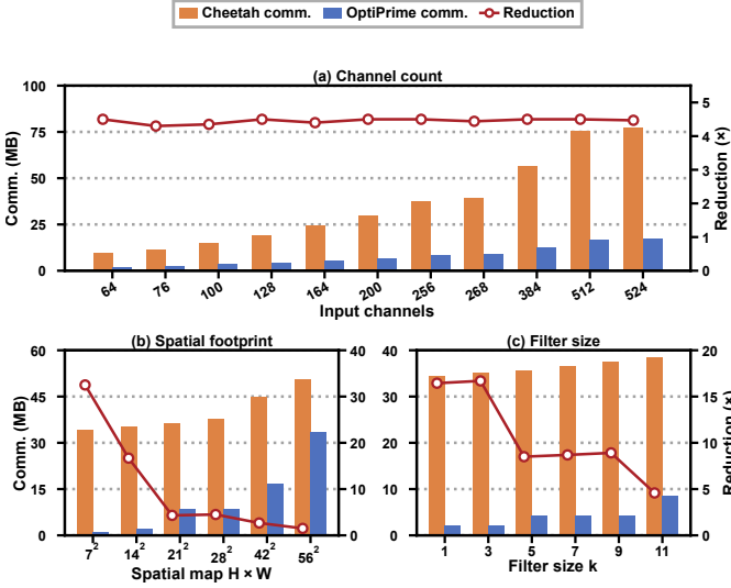
Fig. 21. Performance of OptiPrime under nonideal (a) input-channel count, (b) spatial map size H \times W , and (c) filter size k , with the other dimensions fixed.
