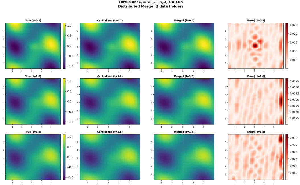
Figure 2: Diffusion equation u_t = D\nabla^2 u : ground truth, centralized fit, Gram merge, and absolute error at three time steps. The white dashed line in the merged column marks the spatial partition boundary ( x = \pi ); Data Holder 1 observes the left half, Data Holder 2 the right. The field smooths as heat diffuses. Centralized and merged reconstructions are identical.
