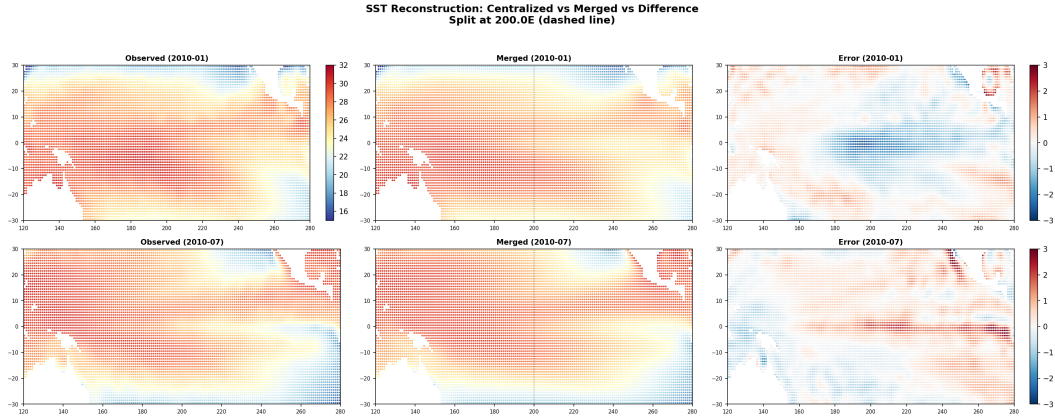
Figure 4: NOAA SST reconstruction: observed temperature fields (left), Gram merge from two data holders split at 200°E (center, white dashed line marks partition), and difference (right). Two months are shown (January and July 2010). The merged reconstruction closely matches the observed field across both data holders’ regions.
