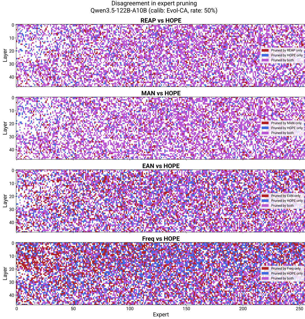
Figure S3: Spatial visualization of disagreement in expert pruning between HOPE and each baseline (Qwen3.5-122B-A10B). Each panel shows an L \times E grid. Disagreement is typically distributed across all layers and experts rather than purely concentrated in certain regions.
