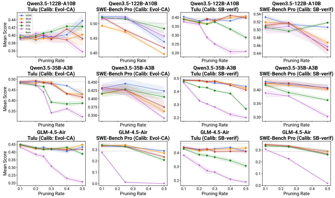
Figure S1: Full performance results across all models and calibration sets. Each row corresponds to a model architecture (Qwen3.5-122B, Qwen3.5-35B, GLM-4.5-Air). Columns alternate between mean Tulu score and SWE-Bench Pro score for each calibration set (Evol-CodeAlpaca and SWE-Bench verified). The dashed gray line indicates the performance of the unpruned base model. HOPE (blue) is competitive or best at all pruning rates, with the cleanest separation at aggressive pruning rates.
