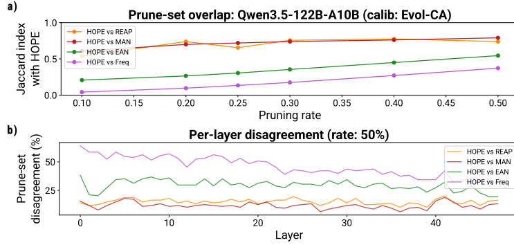
Figure 4: HOPE makes distinct pruning decisions from other baseline methods. a) Overlap between HOPE’s pruning set versus each baseline, as a function of pruning rate (Qwen3.5-122B-A10B). We measure overlap as the Jaccard index, due to the prune-set size varying over different prune rates. b) For the same model and calibration set, the percentage of disagreeing pruned experts (per layer) between HOPE versus other methods at a pruning rate of 50%. Disagreement is distributed across the full network.
