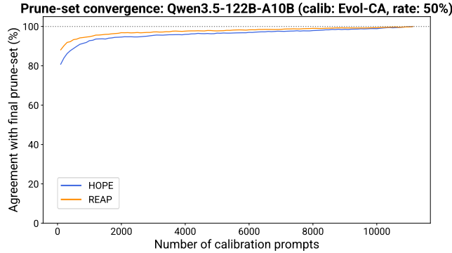
Figure S6: Convergence of pruning decisions with calibration data. We measure the fraction of pruning decisions that agree with the final pruning set (computed from the entire calibration set) as a function of the number of calibration prompts processed. Both HOPE and REAP stabilize within 10k prompts, with HOPE requiring marginally more data to converge due to estimating pairwise (rather than per-expert) statistics. Convergence is shown for 50% pruning on Qwen3.5-35B-A3B with the Evol-CodeAlpaca calibration set.
