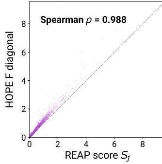
Diagonal of F vs REAP scores (all layers)
