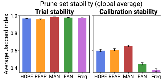
Figure 5: Prune-set stability across calibration sets and trials. a) Jaccard index across independent trials of the same method (averaged over models, pruning rates, and calibration sets). b) Jaccard index between prune-sets produced from different calibration sets: Evol-CodeAlpaca and SWE-Bench verified. Jaccard index is averaged over models, pruning rates, and trials (higher is more stability).
