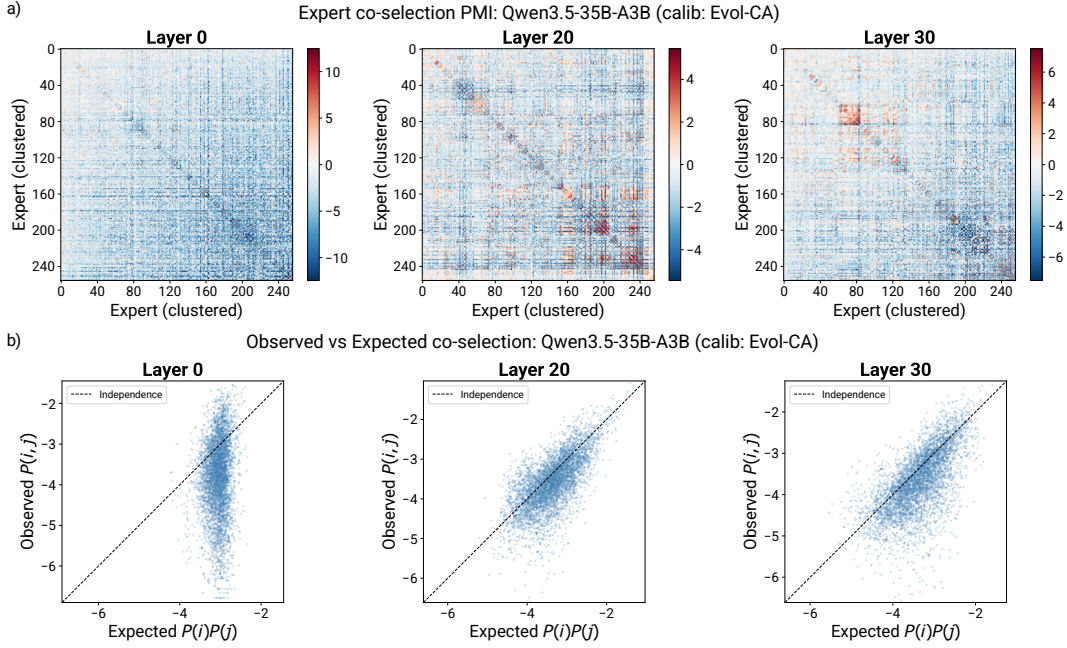
Figure S2: Expert co-selection is highly non-random, which motivates interaction-aware pruning. a) Point-wise mutual information (PMI) between expert pairs. PMI is defined between two experts i, j (within a layer) as PMI(i, j) = \log_2 \frac{P(i, j)}{P(i)P(j)} , where P(i, j) is the fraction of tokens which activate both experts, and P(i) is the fraction of tokens which activate only one expert i . We show PMI between experts at three different layers of Qwen3.5-35B-A3B. Positive values (red) indicate experts are co-selected more often than expected due to independent chance; negative values (blue) indicate experts are co-selected less often (mutual exclusion). b) Observed co-selection probability P(i, j) versus independence expectation P(i)P(j) . Under completely independent routing, all points should lie on the diagonal. Any substantial deviation (which is especially pronounced at layer 0) demonstrates that experts operate in cooperative groups.
