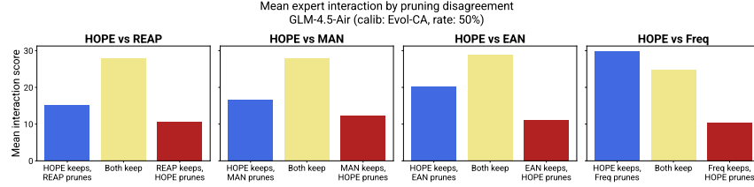
Figure 3: HOPE preferentially retains experts with stronger cooperative structure. For each baseline, we classify experts by disagreement (kept only by HOPE, kept only by the baseline, or kept by both). Experts kept by HOPE tend to have higher cooperative score (measured as the mean F score with HOPE-retained experts).
