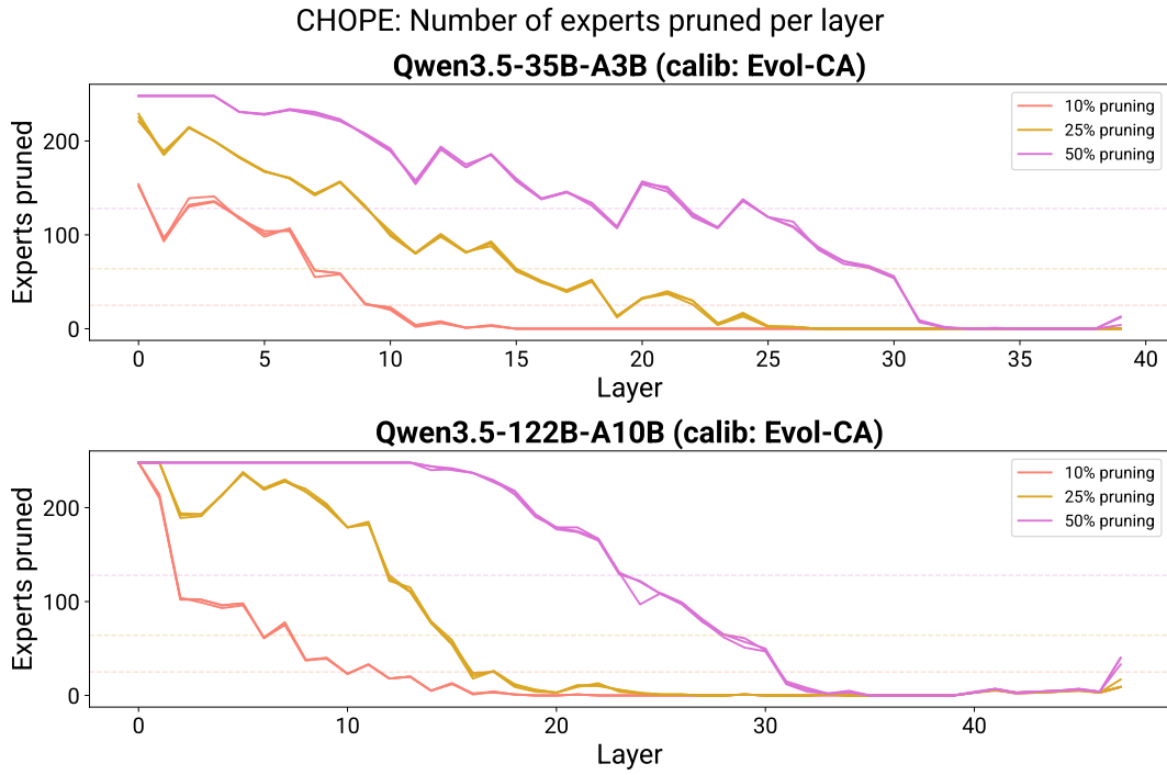
Figure S7: Non-uniform expert pruning allocation by CHOPE (cross-layer HOPE). Each line indicates the number of experts pruned per layer (3 independent trials for each pruning rate); dashed horizontal lines indicate the uniform budget (used by per-layer HOPE).
