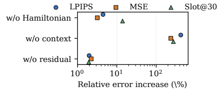
Figure 9: Compact OBJ3D ablation summary. The plot shows relative error increases when the physical, context, or residual pathway is removed.
