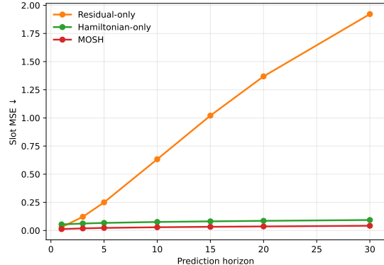
Figure 10: Physion slot error over the prediction horizon. The complete model remains lowest throughout the rollout.
