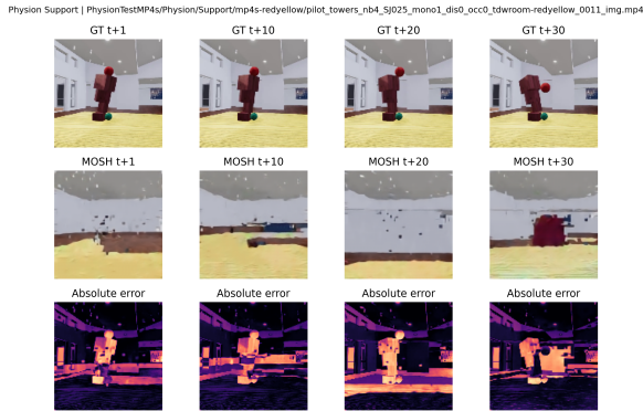
Figure 11: Physion qualitative transfer. Ground truth, MOSH prediction, and absolute reconstruction error are shown at horizons 1, 10, 20, and 30. Pixel quality is limited by the frozen STEVE decoder; the experiment is primarily a slot-dynamics transfer test.
