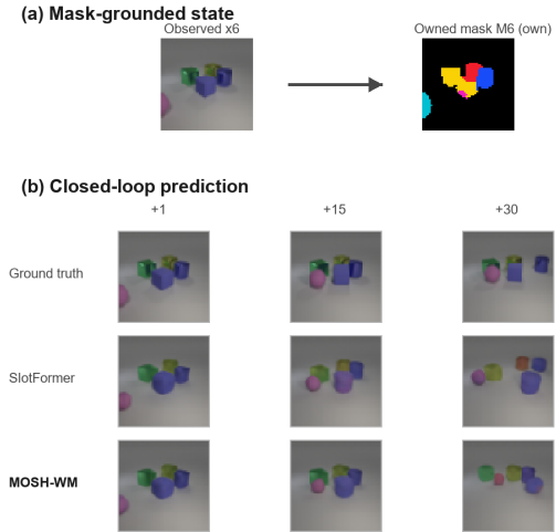
Figure 1: Mask grounding and long-horizon prediction on OBJ3D. Owned masks expose object support. SlotFormer matches the immediate future but drifts over closed-loop rollout; MOSH-WM better preserves object identity and scene layout.
