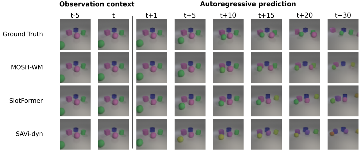
Figure 3: Long-sequence prediction on OBJ3D. Two observation frames and six future frames are shown at a larger scale than a full-frame strip. All rows use the same six-frame context and independently exported 30-frame closed-loop predictions. Under repeated feedback, MOSH-WM better retains object identity, color, and relative layout.
