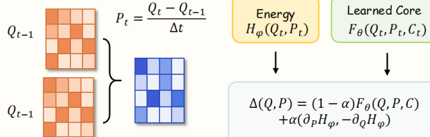
Figure 2: MOSH-WM pipeline. A frozen SAVi interface supplies visual slots and decoded masks. Mask-owned pooling extracts Q , raw temporal differences provide P , and causal slots provide C . The SOFT-HAMILTONIAN update propagates (Q, P) ; a gated composer and bounded spatiotemporal residual return to decoder-compatible slot space. Dashed arrows denote direct state propagation and autoregressive context update.
