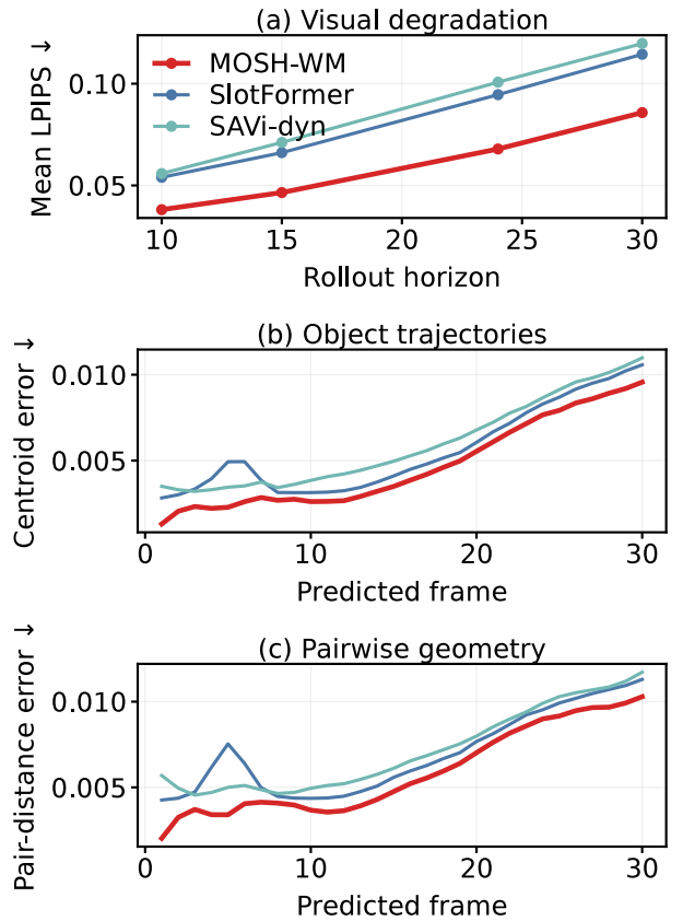
Figure 5: OBJ3D closed-loop error accumulation. (a) Mean LPIPS over increasing horizons. (b) Per-frame centroid error. (c) Per-frame pairwise-distance error. All curves use the same six observations.
