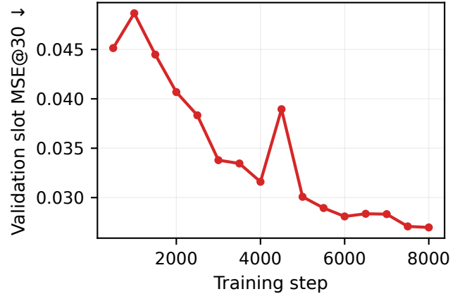
Figure 7: Validation Slot@30 during the main OBJ3D training run. The curve is used for checkpoint selection.
