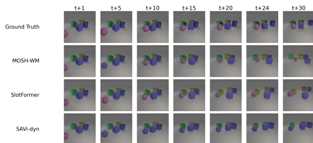
Figure 8: Additional OBJ3D 6-to-30 rollout on test video 125. Columns show future horizons and rows compare ground truth with three predictors under the same closed-loop protocol.
