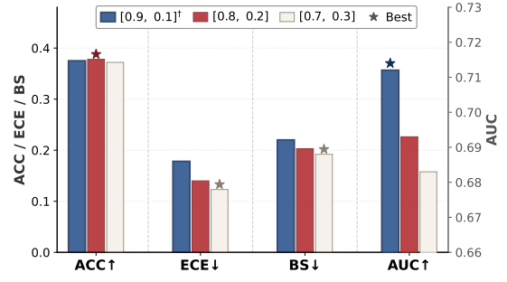
Figure 8: Sensitivity study on stake margin thresholds. The default setting uses the clipping range [0.9, 0.1], and we additionally evaluate [0.8, 0.2] and [0.7, 0.3]. Stars (*) indicate the best value within each metric. Left axis: ACC, ECE, BS; right axis: AUC.
