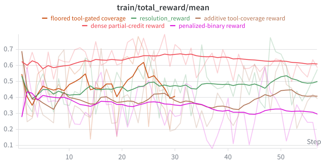
Figure 3: Reward trends across designs on the smaller proxy policy ( train/total_reward/mean ). Each curve is that run’s own reward, so the vertical scales differ and only the trend (shape and stability) is meaningful, not the absolute level. The final gated-coverage reward ( resolution_reward , green) trends up and stays stable; the penalized-binary reward (magenta) trends down; the additive and floored variants are noisy and flat-to-declining. The dense partial-credit reward (red) is highest only because partial credit inflates its own scalar (reward hacking), not because resolution is better.
