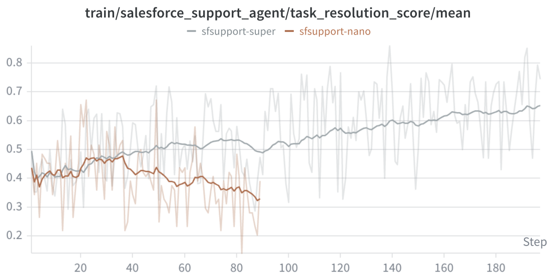
Figure 4: The same final gated-coverage reward at two model scales ( train/salesforce_support_agent/task_resolution_score/mean ). On the Super-120B policy ( sfsupport-super , gray) task resolution improves steadily to \approx 0.65 over \approx 200 steps; on the smaller proxy/Nano policy ( sfsupport-nano , red) it peaks near step 30 ( \approx 0.47 ) and then collapses to \approx 0.33 . Dark = smoothed, light = raw per-step.
