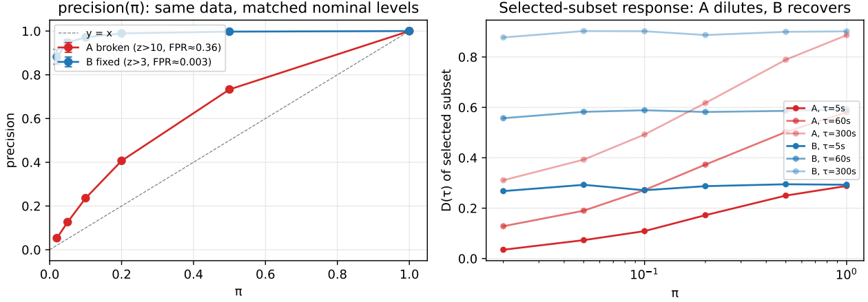
Figure 4: Two detectors at matched nominal strictness on identical data. Left: at \pi = 0.02 , A attains precision 0.053 while B attains 0.882. Right: the response curve measured on each detector’s selected subset, as a function of \pi : A’s estimate drifts with the composition of its own selection; B’s is stable.
