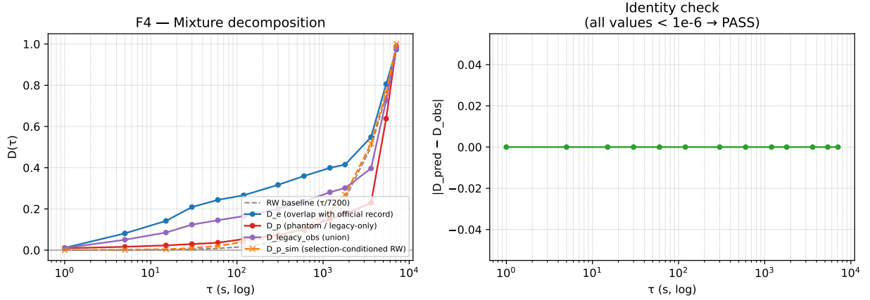
Figure 2: Left: the detected dataset’s curve decomposed into its true-event component D_E , its phantom component D_P , and the exact mixture, with the unconditional random-walk baseline and the selection-conditioned null for D_P . Right: identity (3) verified to machine precision.
