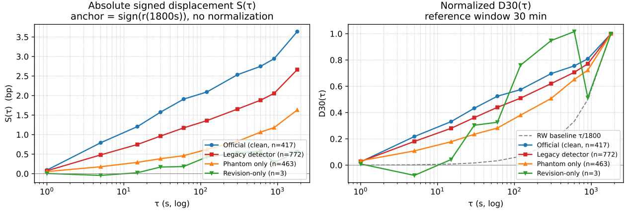
Figure 3: Same price windows, two label sets, two estimators. Left: denominator-free signed displacement S(\tau) in bp. Right: normalised D_{30}(\tau) with its random-walk baseline \tau/1800 . Official n=417 , detected n=772 , phantom-only n=463 . The revision-only control is plotted at n=3 and is not interpretable; only 3 of the 17 calendar-identified control windows have price coverage (App. C). Under terminal normalisation (App. D) the official/detected ordering is reversed relative to the left panel.
