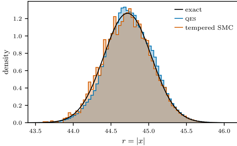
Figure 8: Reconstructed radial posterior at D = 10^4 against the exact shell r = \tau\chi_D , for a single run at the default working point. Both methods pool every weighted particle from every level of the path: QES with the level-volume quadrature weights of Appendix C.3, tempered SMC with deterministic-mixture balance weights over its temperatures. The pooled Kish ESS is 4.8 \times 10^5 for QES and 6.9 \times 10^3 for tempered SMC.
