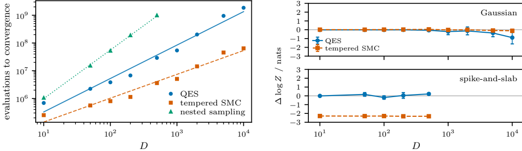
Figure 2: Cost and accuracy order the three methods oppositely. Left : evaluations to convergence against dimension on the Gaussian, each method run to its own criterion at N = 1000 , with a fitted power law \text{evals} = CD^\alpha . The cost exponents are \alpha = 0.86 for tempered SMC, 1.21 for QES and 1.75 for nested sampling. Right : evidence bias on a shared symmetric axis, Gaussian and spike-slab. Nested sampling counts likelihood evaluations, the other two count gradients, so cost is not exactly comparable.
