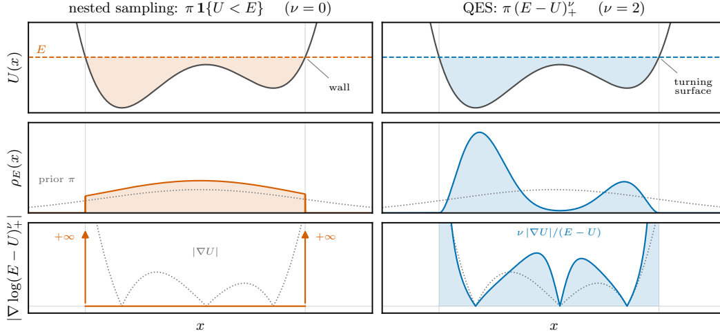
Figure 1: Illustration of QES against nested sampling, on a one-dimensional asymmetric double well (unit Gaussian prior). Top : the energy landscape U with the level E as a waterline. Middle : the profile of \rho_E under the two choices of \nu . Bottom : the resulting score of \rho_E ; for \nu > 0 it is a smooth informative gradient throughout the interior of the level set, vanishing only at stationary points of U . The dotted reference is the magnitude of the gradient of U .
