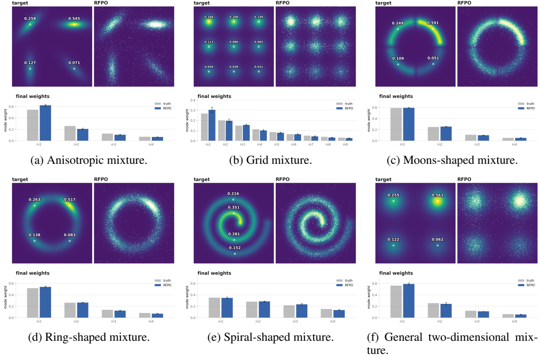
Figure 3: Results on six synthetic two-dimensional target distributions with diverse geometries after 3,000 training rounds. In each subfigure, the upper-left panel shows the target density, where the white markers indicate the predefined modes and the annotated values denote their ground-truth probability masses. The upper-right panel overlays samples generated by the learned RFPO policy on the target density. The lower panel compares the ground-truth mode weights (gray) with those estimated from the RFPO samples (blue), with error bars indicating variability across repeated runs. Across the different geometries, RFPO covers multiple high-density regions, follows nonlinear ridge structures, and closely reproduces the unequal probability masses assigned to the modes.
