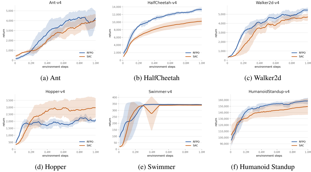
Figure 2: Learning curves on six continuous-control tasks. Each curve represents the average return over 5 random seeds, with the shaded area indicating one standard deviation from the mean.
