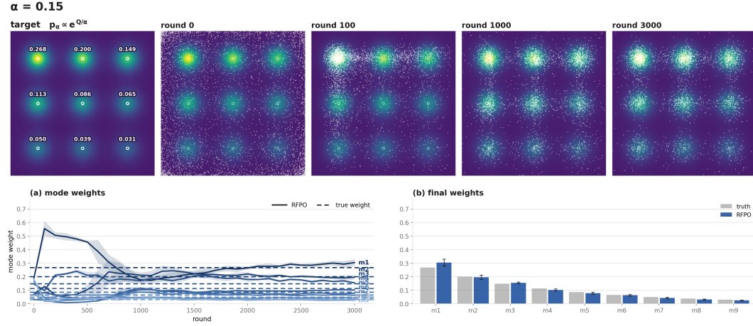
Figure 5: RFPO on the grid mixture target distribution.
