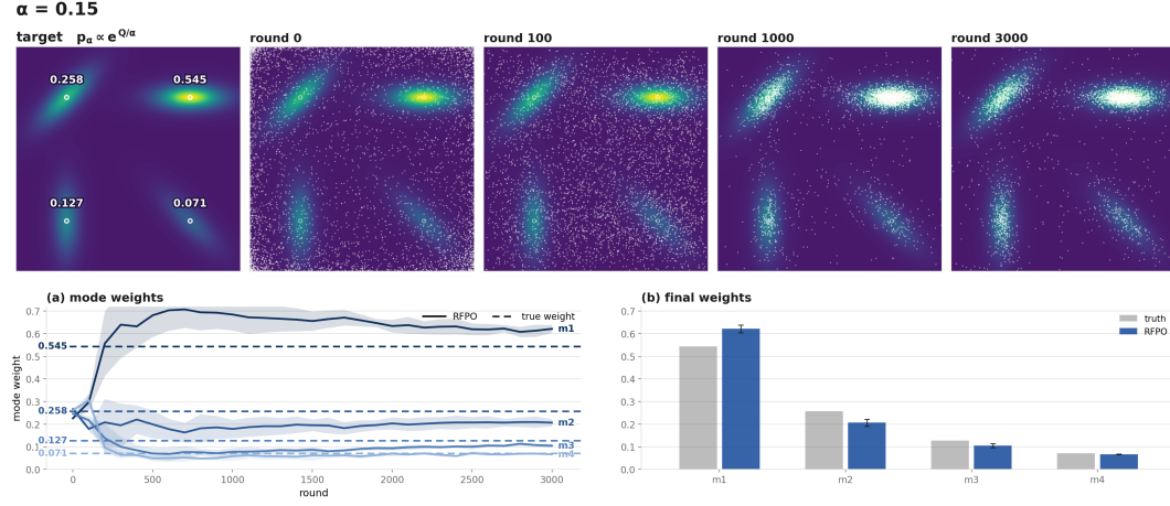
Figure 4: RFPO on the anisotropic mixture target distribution.
