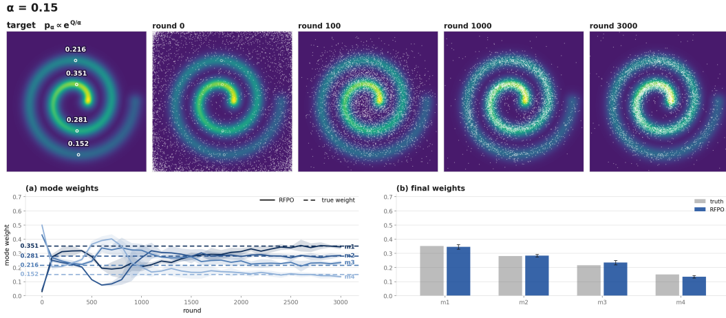
Figure 8: RFPO on the spiral-shaped target distribution.
