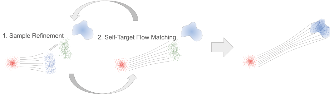
Figure 1: Overview of RFPO. Shaded regions illustrate the target distribution p_\alpha(\cdot | s) . Red dots denote Gaussian base samples x_0 , blue dots denote actions a_1 generated by integrating the flow ODE, and green dots denote refined actions a'_1 . Q-guided sample refinement updates the flow-generated actions toward the target distribution (left). The refined actions are paired with their corresponding original base samples to train the policy through self-target flow matching (center). The curved arrows indicate repeated alternation between these two processes. The learned flow policy is shown approximating the target distribution after repeated updates (right).
