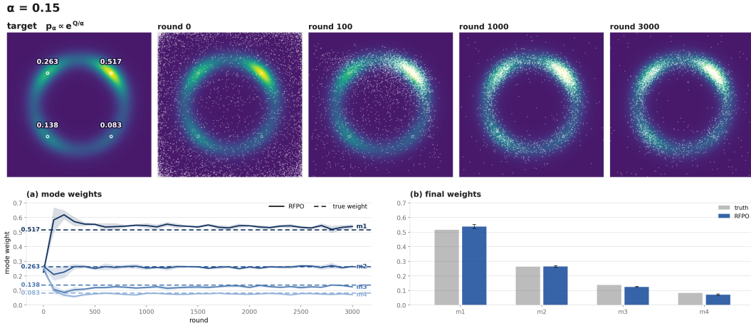
Figure 7: RFPO on the ring-shaped target distribution.
