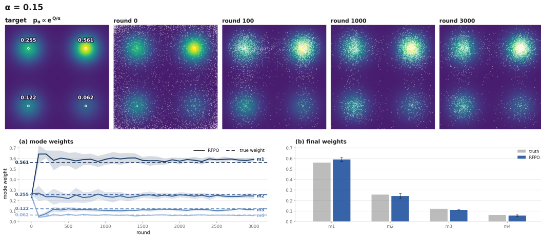
Figure 9: RFPO on the general two-dimensional mixture target distribution.
