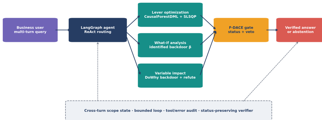
Figure 4: Conversational architecture. Tools invoke the causal engine; F-DACE and the verifier retain decision authority over the returned status.
