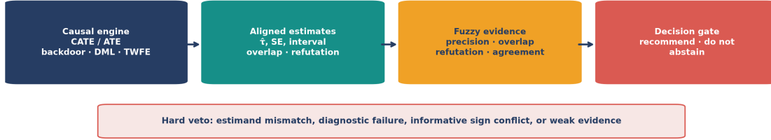
Figure 3: F-DACE consumes aligned engine outputs and applies a non-compensatory veto before recommendation or abstention.
