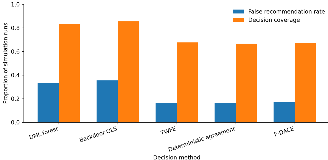
Figure 5: False-recommendation rate and decision coverage across six synthetic conditions. Lower false recommendation and higher coverage are desirable but competing objectives.
