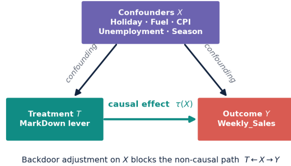
Figure 1: Assumed causal graph of the engine. Backdoor adjustment on X blocks the spurious path T \leftarrow X \rightarrow Y .
