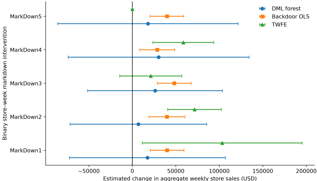
Figure 6: Store-week estimates and 95% intervals. The spread is evidence consumed by F-DACE, not a set of interchangeable estimates to average.
