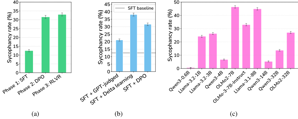
Figure 3: Sycophantic agreement rate of different OLMo-3-7B post-training stages and other post-trained models from OLMo2, Qwen3, and Llama-3.1/3.2 families. (a) For OLMo-3-7B post-training, the sycophantic agreement rate more than doubles after DPO training and persists through RLVR. (b) For the OLMo-3-7B DPO stage, training only on GPT-judged data (SFT + GPT-judged) leads to a lower sycophantic agreement rate than training only on delta learning data (SFT + Delta learning). The gray line is the baseline sycophantic agreement rate of the SFT stage. (c) Sycophantic agreement rates of ten post-trained models from the OLMo2/3, Qwen3, and Llama-3.1/3.2 families.
