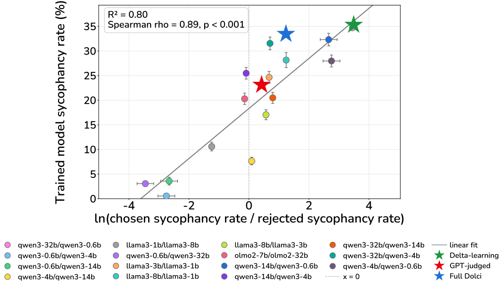
Figure 7: Figure 4a with a full legend included, labeled as “{chosen model}/{rejected model}”.
