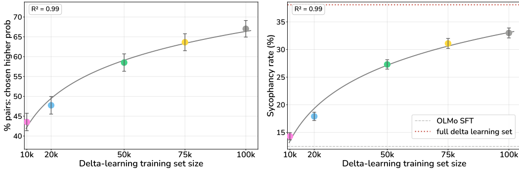
Figure 6: Sycophancy scales with training set size similarly to preference learning itself. Models are trained with DPO on n randomly selected datapoints from the delta learning dataset. (a) Preference learning performance, measured as the percentage of preference pairs where the chosen response receives higher probability. (b) The sycophantic agreement rate follows a closely matching power law.
