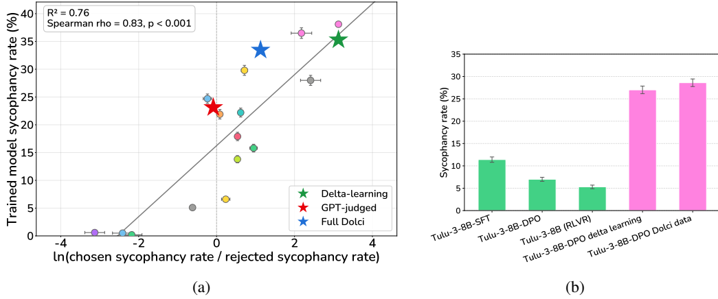
Figure 4: The log-ratio of the chosen and rejected models’ sycophancy rates predicts the student model’s sycophancy across two base models and training pipelines. (a) We train 15 DPO models using different pairs of teacher models from the same families, and we find a strong correlation between the log-ratio of the chosen and rejected models’ sycophancy and the sycophancy of the trained model. The correlation holds even when multiple models are used to generate the chosen responses and rejected responses, as in the GPT-judged setting. Legend with all model pairs in Appendix C. (b) In Section 3.4, we benchmark the sycophancy rates of the official Tulu-3-8B checkpoints , for which the DPO data was chosen through the GPT-judged method. We then retrain DPO on delta learning Tulu data and on Dolci-Instruct-DPO-7B , and we find that models trained on the delta learning principle are significantly more sycophantic than the original checkpoints, matching the results from the OLMo 3 pipeline.
