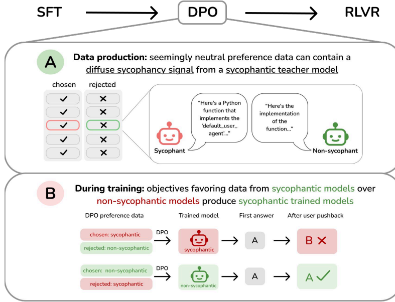
Figure 1: Sycophantic agreement can transfer through seemingly neutral preference data during training under contrastive optimization objectives. (A) During data production, a more sycophantic model producing chosen responses and a less sycophantic model producing rejected responses generate similar, innocuous-looking completions. This means that sycophancy is not easily detectable on the datapoint level, but a diffuse sycophancy signal emerges on the dataset level. (B) During training, contrastive preference optimization methods transfer the chosen model’s sycophancy to the student. A model trained on data from a sycophantic chosen model displays sycophantic agreement, while a model trained on data from a non-sycophantic chosen model does not.
