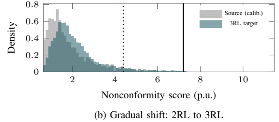
Fig. 8. Source-calibration and 3RL-target score distributions. Dotted and solid lines mark \tau_{\text{CP}} and \tau^* , respectively. Target miss rates are 7.36% (abrupt) and 5.62% (gradual).
