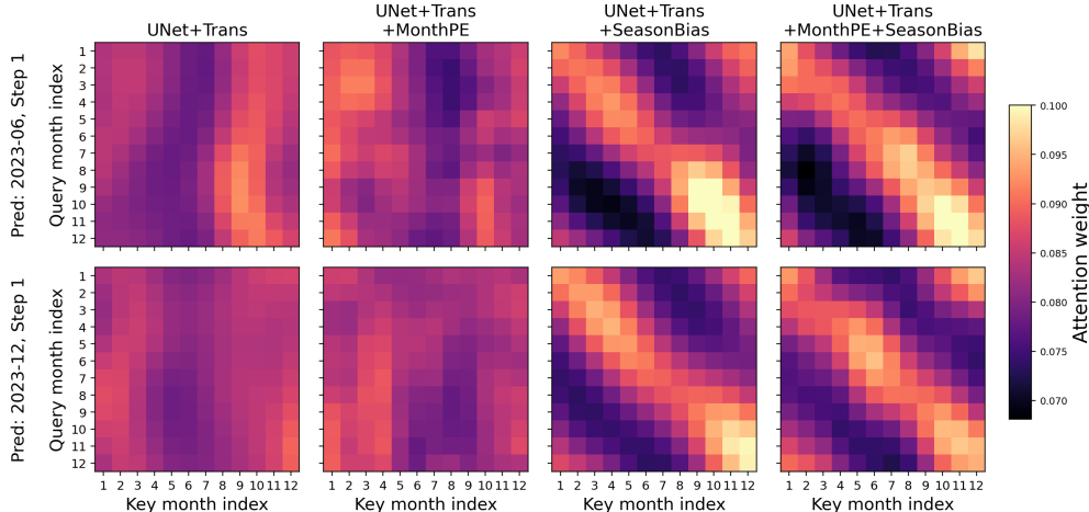
Figure 4: Temporal attention heatmaps of UNet+Trans variants for representative forecast cases. Columns correspond to the baseline model, the model with MonthPE, the model with SeasonBias, and the model with both MonthPE and SeasonBias. Rows show predictions for June and December 2023 at the first autoregressive step.
