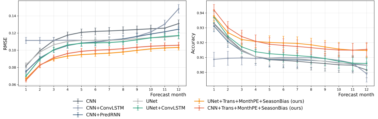
Figure 2: Comparison of multi-horizon forecasting performance across baseline and Transformer-based models over a 12-month autoregressive prediction horizon. The left panel shows the RMSE for continuous SIC prediction, while the right panel shows the classification accuracy for categorical SIC prediction. Markers denote the mean over repeated runs, and error bars represent the standard error.
