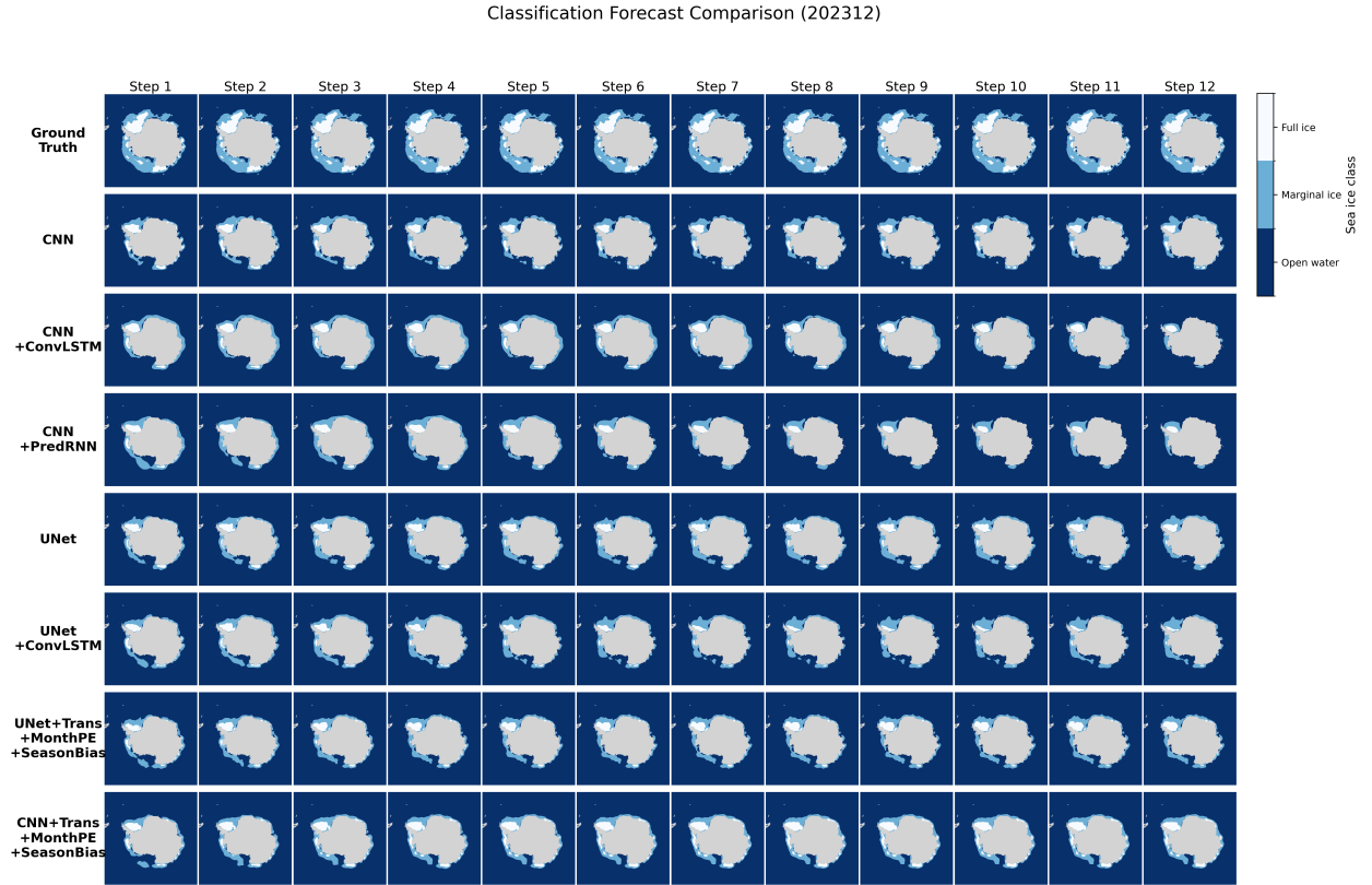
Figure 6: Qualitative comparison of multi-step sea ice classification forecasts initialized in December 2023. Each column represents a forecast lead time from step 1 to step 12, and each row corresponds to the ground truth or one forecasting method. The three classes denote open water, marginal ice, and full ice.
