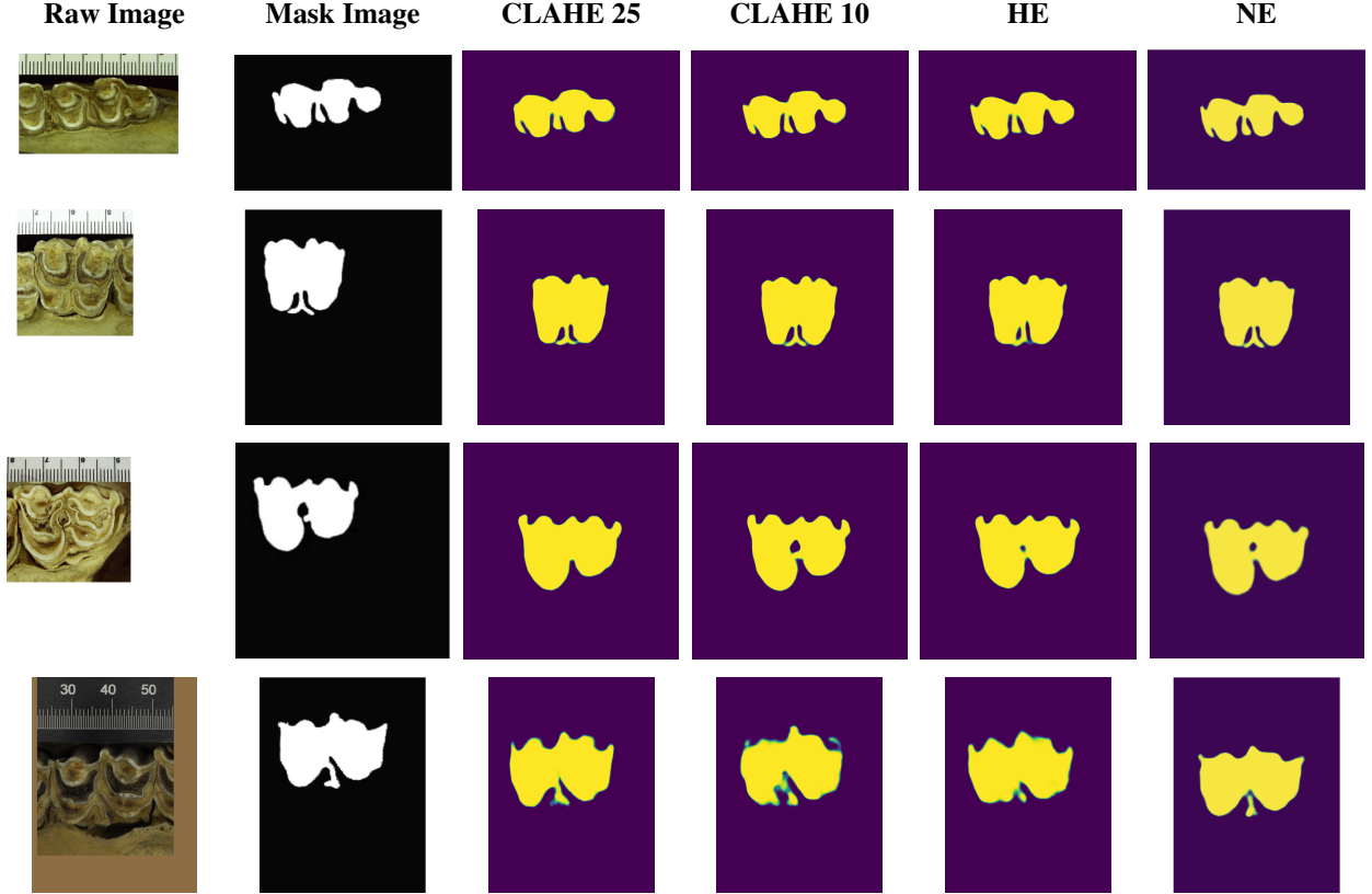
Figure 4. Example Raw Images (including whitespace) and ground-truth Mask Images as well as inferred heatmaps by SegFormer MiT-B3 using different histogram equalization techniques. Yellow represents regions with high ( \sim 1 ) likelihood of being part of the tooth; purple represents low likelihood. Best viewed in color.
