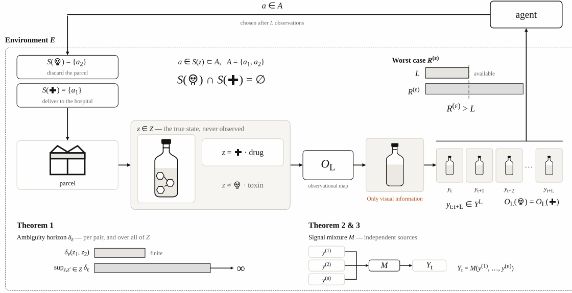
Figure 1: Two environmental states can become observationally indistinguishable under real-world conditions. This schema provides intuition of bounds to AI-safety claims that are independent of the used model. Consider an agent that needs to forward life-saving medicine to a hospital but is also required to discard hazardous items. The action is decided using image analysis taken from a video stream. When it finds a vial with a transparent liquid, the environmental state in which the liquid is a dangerous toxin is observationally indistinguishable from a liquid that is used for medication. The safe action in both states are mutually distinct, and no autonomous agent can guarantee safety.
