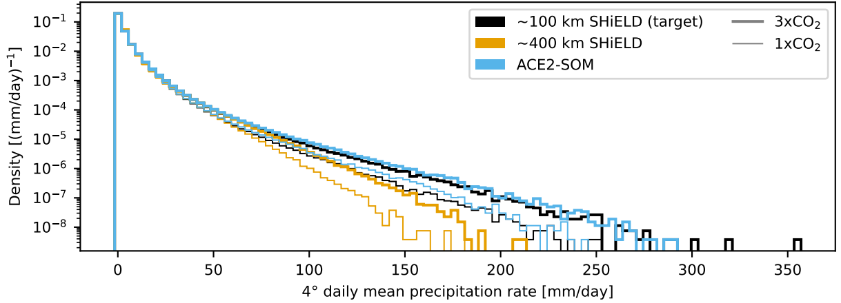
Figure 5: Extreme precipitation in ACE2-SOM. Daily precipitation distributions from 50-year samples of reference slab-ocean-coupled \sim 100 km and \sim 400 km SHiELD simulations, and ACE2-SOM for present-day and unseen 3\times\text{CO}_2 climates, regridded to a common 4^\circ Gaussian grid. ACE2-SOM reproduces the target \sim 100 km model’s extreme-precipitation frequency and its sensitivity to \text{CO}_2 -induced warming. Adapted from Fig. 6 of [115].
