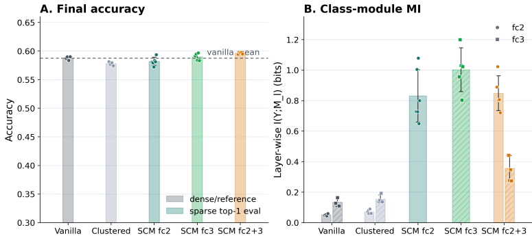
Figure 3: Measures of accuracy and MI of the same CNN model after training on ImageNet-100 CMC. A: The accuracies of our method, clustered baseline from [8] and without modularization. Here, the accuracy of our method corresponds to the top-1 accuracy while other methods are evaluated on dense accuracies. B: the MI between the favored module and the input class.
