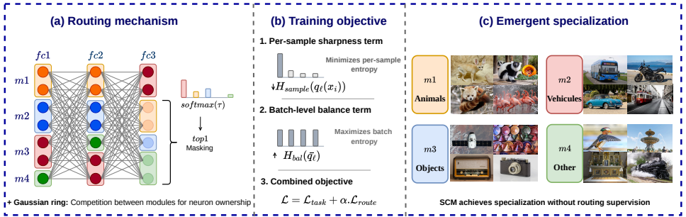
Figure 1: Overview of Sparse Competitive Modules. (a) A routed layer is partitioned into modules. For each input, module activation energies are converted into routing probabilities, and a hard top-1 mask keeps only the selected module active. (b) The routing objective combines a per-sample sharpness term, which encourages confident module selection, with a batch-level balance term, which prevents collapse by encouraging all modules to be used. (c) Without module-level or semantic supervision, the resulting routing assignments become class-informative, where visually related classes tend to share dominant modules.
