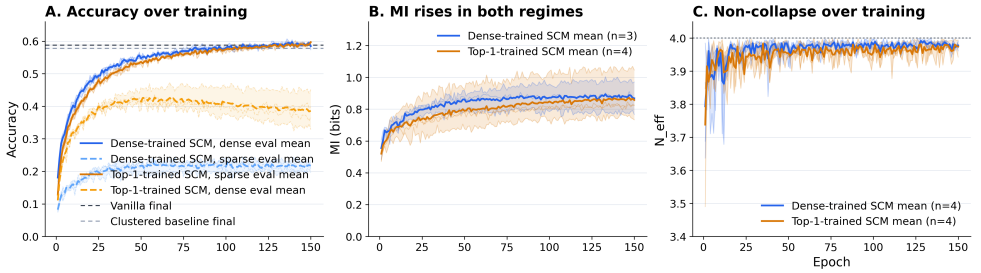
Figure 4: Evolution of metrics during training on ImageNet-100 CMC. A. The top-1 accuracies of our method (SCM) compared to no clustering (Vanilla) and the method from [24] (Clustered); in dotted lines are the opposite evaluations compared to training: the dense training is on sparse eval, and the sparse training is on dense eval. Both regimes perform better when evaluated like training, but sparse training is better on dense than dense on sparse eval. B. The evolution of MI between our method trained in sparse and dense training. C. The evolution of the effective number of modules at the end of training. The trainings on our method converge on N_{eff} = 4 meaning all modules are used evenly.
