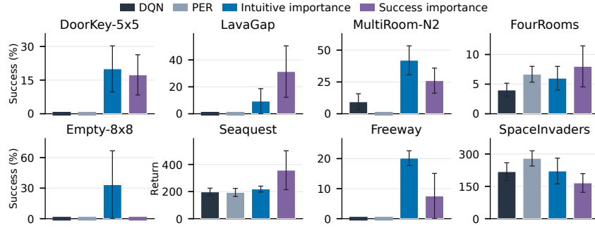
Figure 5: RL with Jev-Rewighted Replay. MiniGrid 10k and Atari 50k endpoints, mean \pm SEM across three training seeds. Tasks with zero performance for all four methods are omitted.
