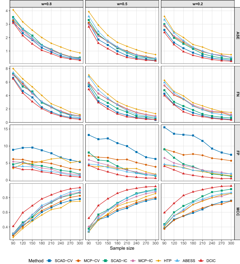
Figure 9: Performance metrics under Setting 2 with an increasing sample size. The suffix “-CV” indicates tuning by 10-fold cross-validation. The suffix “-IC” indicates tuning by information criterion.
