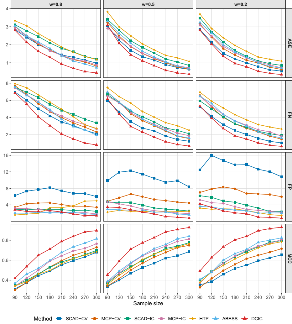
Figure 4: Performance metrics under Setting 3 with an increasing sample size. The suffix “-CV” indicates tuning by 10-fold cross-validation. The suffix “-IC” indicates tuning by information criterion.
