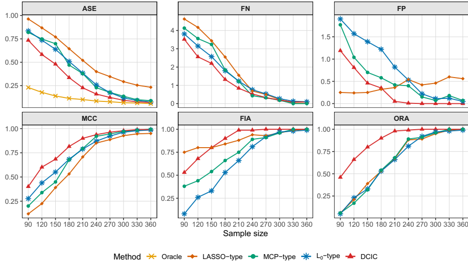
Figure 5: Performance metrics under Fourier truth with an increasing sample size.
