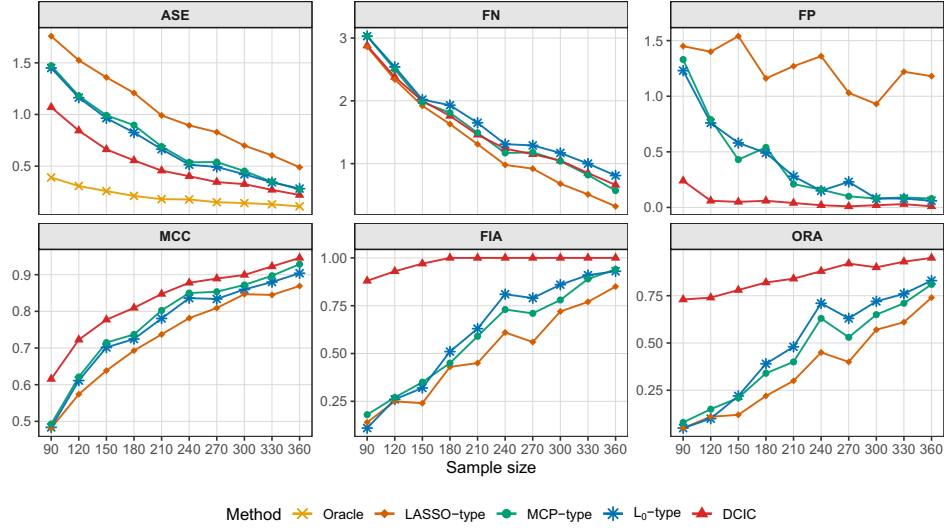
Figure 6: Performance metrics under spline truth with an increasing sample size.
