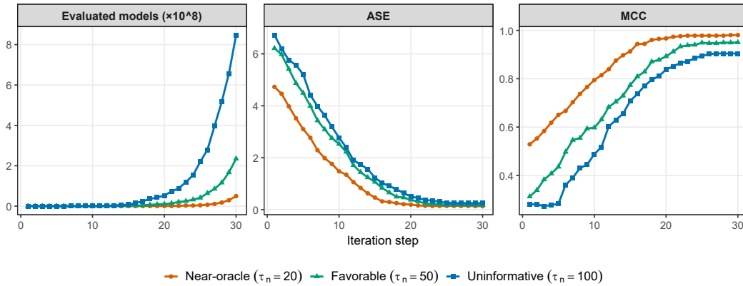
Figure 10: Pathwise computation–statistics trade-off under different ranking informativeness. The curves are averaged over 100 replications.
