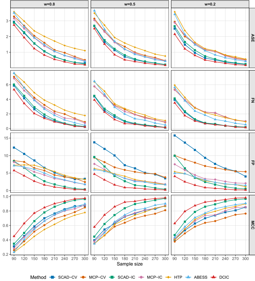
Figure 8: Performance metrics under Setting 1 with an increasing sample size. The suffix “-CV” indicates tuning by 10-fold cross-validation. The suffix “-IC” indicates tuning by information criterion.
