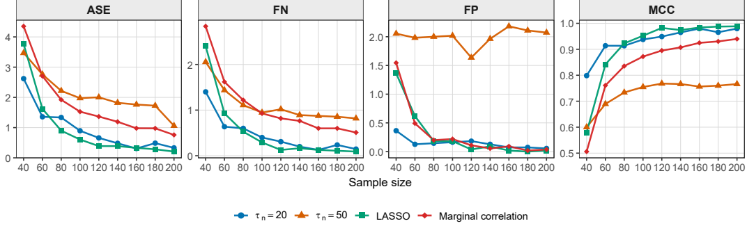
Figure 12: Performance of different ranking procedures under a moderately correlated AR(1) design.
