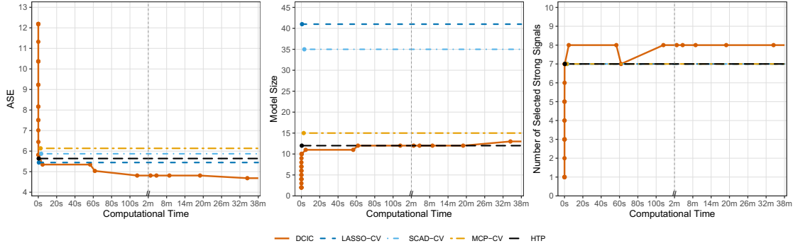
Figure 2: Computation–statistics trade-off under a misspecified dense-signal model with n = 200 , p = 1000 , \sigma = 2 , \rho_{\text{in}} = \rho_{\text{out}} = 0.7 , and w = 0.5 . The coefficient vector contains 10 strong, 50 moderate, and 940 weak signals. The variables are partitioned into ten equal-sized blocks, each containing one strong and five moderate signals. Signal magnitudes are drawn independently from \text{Unif}(1, 1.3) , \text{Unif}(0.2, 0.4) , and \text{Unif}(0, 0.1) , respectively, with independent random signs.
