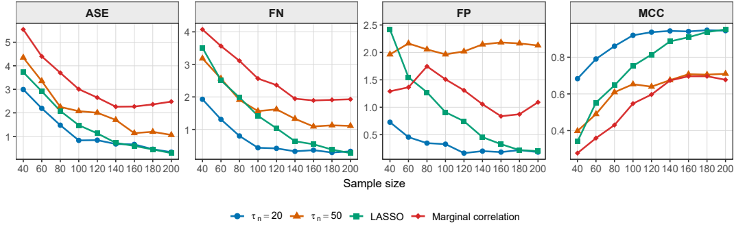
Figure 11: Performance of different ranking procedures under a strongly correlated design.
