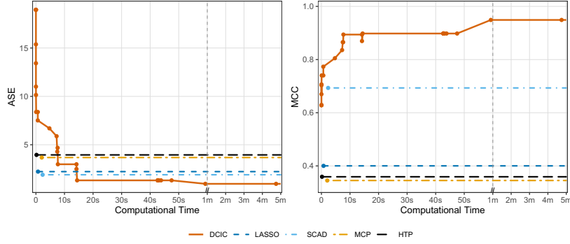
Figure 1: Computation–statistics trade-off under a well-specified, strongly correlated design with n = 200 , p = 1000 , s^* = 20 , \sigma = 2 , \rho_{\text{in}} = \rho_{\text{out}} = 0.9 , and w = 0.5 .
