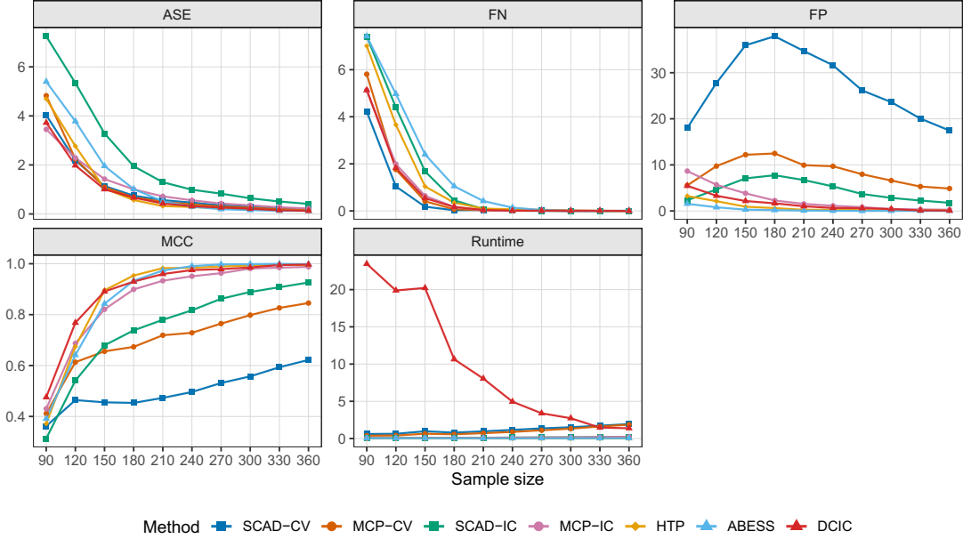
Figure 14: Performance under the AR(1) design with \Sigma_{ij} = 0.6^{|i-j|} as the sample size increases. The suffix “-CV” denotes tuning by 10-fold cross-validation, whereas “-IC” denotes tuning by an information criterion.
