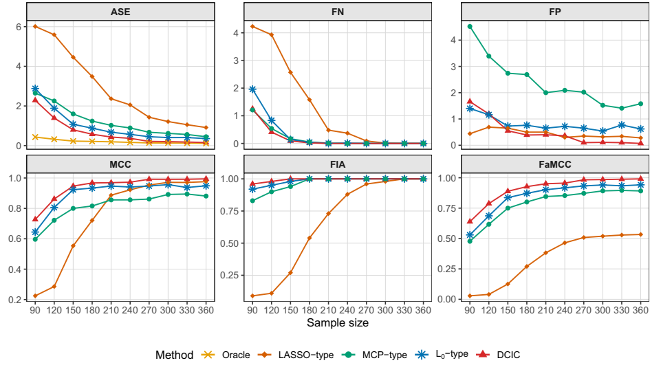
Figure 7: Performance metrics under Haar truth with an increasing sample size.
