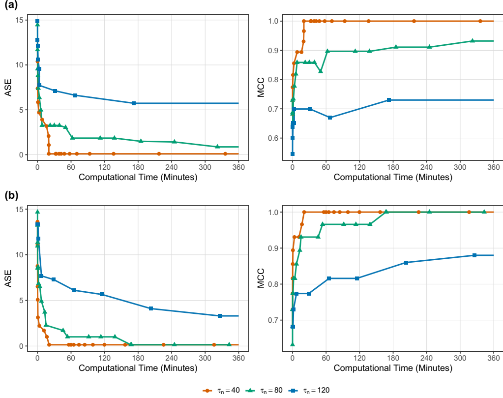
Figure 13: Representative large-scale runtime illustration of the pathwise computation-statistics trade-off, with n = 200 , p = 5000 , and s^* = 20 . The curves report ASE and MCC against accumulated computational time under different rank envelopes \tau_n . Panel (a) corresponds to the strongly correlated design in Setting 1 of Section 6.1, with \rho_{\text{in}} = \rho_{\text{out}} = 0.9 and w = 0.5 ; panel (b) corresponds to an AR(1) design with \Sigma_{ij} = 0.6^{|i-j|} .
