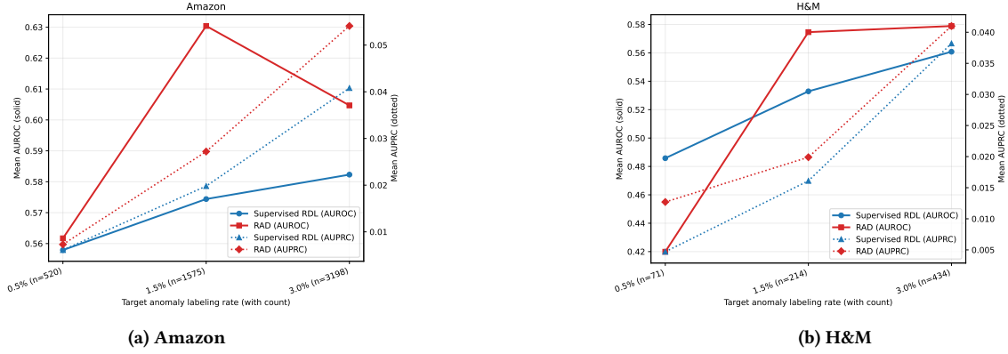
Figure 4: Label-prevalence sensitivity for unexpected-churn detection. AUROC uses the left axis and AUPRC the right axis for target prevalences of 0.5%, 1.5%, and 3.0%; counts show retained positives.
