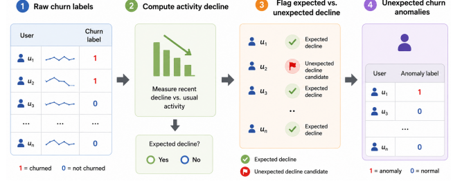
Figure 2: Unexpected-churn filtering. Churned users with an expected prior activity decline are removed; remaining churned users are treated as unexpected-churn anomalies.
