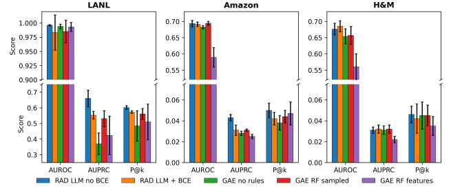
Figure 3: Rule-construction and structure-reconstruction ablations across datasets over 10 seeds. Bars show means and error bars show standard deviations. The y-axis is broken to separate AUROC from smaller AUPRC and P@k values.
