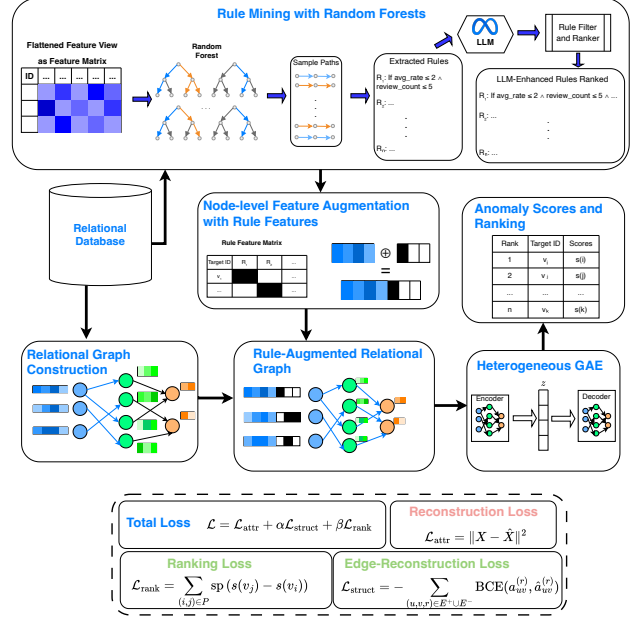
Figure 1: Overview of RAD. A database is represented by a flattened view for rule mining and a heterogeneous graph for representation learning. Random-forest paths are refined into predicates, converted into binary features, and injected into nodes before heterogeneous graph encoding. The model produces anomaly scores and ranks target nodes.
