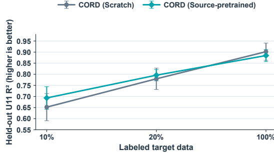
Figure 8: Engine R^2 under the same matched 400-update protocol as Figure 4. Points and error bars show mean \pm sample SD over five seeds.
