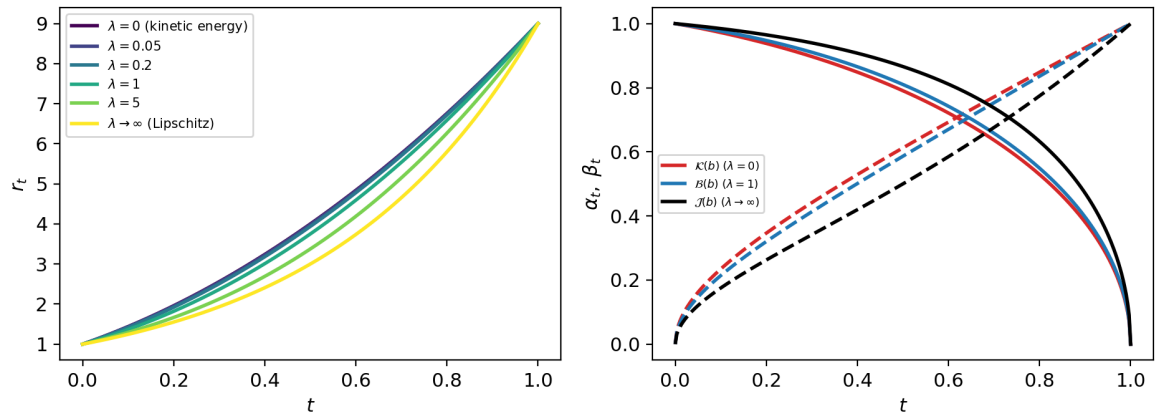
Figure 1: Left : Optimal eigenvalue (r_t)_{t \in [0,1]} for different regularization strength. Right : Optimal schedulers (\alpha_t)_{t \in [0,1]} (continuous) and (\beta_t)_{t \in [0,1]} (dashed) for the three objectives \mathcal{K}, \mathcal{B} and \mathcal{J} .
