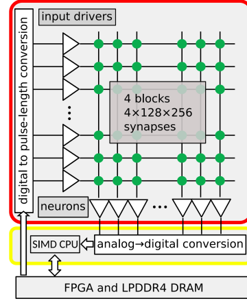
Fig. 1: Internal structure of the BSS-2 ASIC, with input drivers (triangles on the left), neurons (triangles at the bottom), and synapses (green dots) [13].
