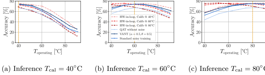
Fig. 7: Validation accuracy versus operating temperature for different training approaches under three hardware calibration conditions. Each subplot represents inference using one calibration created at T_{\text{cal}} .
