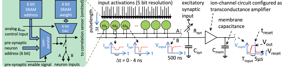
Fig. 2: Principle of analog matrix-vector multiplication on BSS-2 [13].
