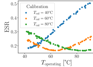
Fig. 6: Error-to-signal ratio over operating temperature T_{\text{operating}} for each calibration.
