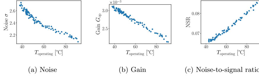
Fig. 5: Temperature-dependent behavior of noise (left) and gain (middle) and noise-to-signal ratio (right).
