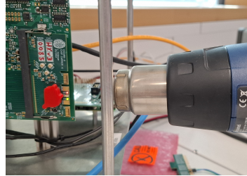
Fig. 4: Experiment setup for temperature measurements with BSS-2.
