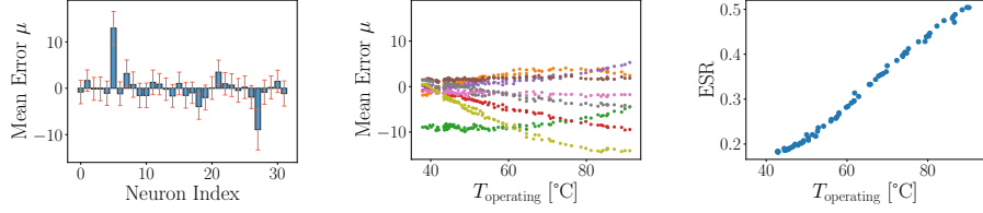
(a) Mean and standard deviation of per-neuron error for a subset of 32 neurons ( T_{\text{operating}} = 40^{\circ}\text{C} ). (b) Per-neuron mean error over temperature for a subset of 8 neurons (each color represents one neuron). (c) Error-to-signal ratio over temperature (described in section 3.2).
