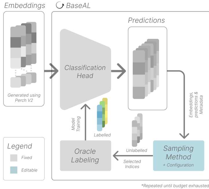
Fig. 1: Active learning loop showing fixed and editable components.
