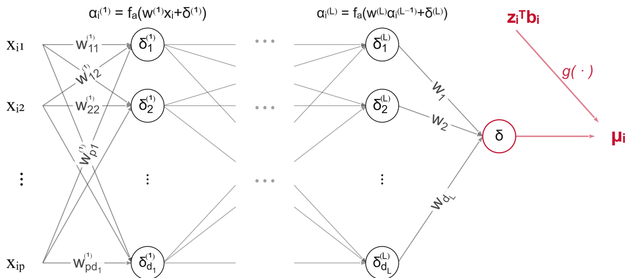
Figure 1: The architecture of a multi-layer NMM.
