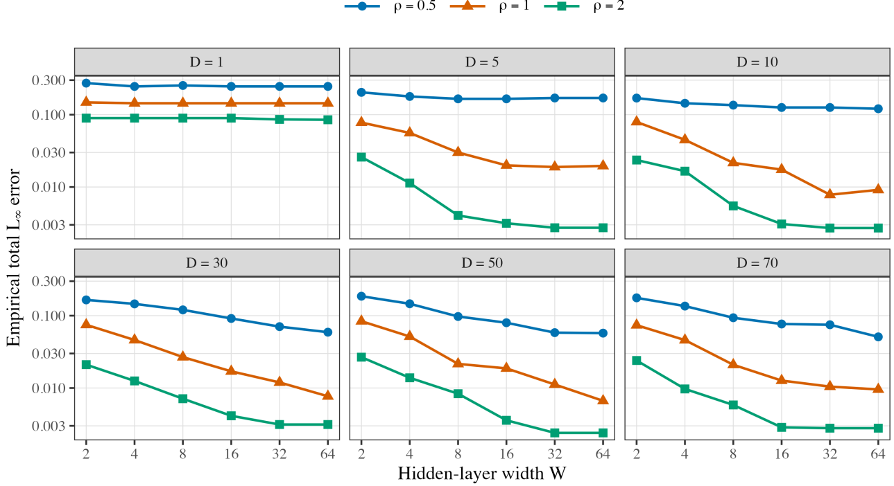
Figure 1. Total approximation error as a function of the common hidden-layer width.
