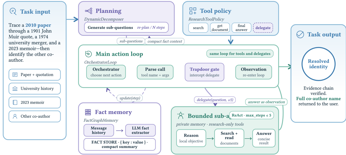
Figure 8: Trapdoor: bounded research behind a delegated tool call. A synthesized delegate capability is intercepted by OrchestratorLoop, which runs a bounded subagent and writes extracted facts into FactGraphMemory.
